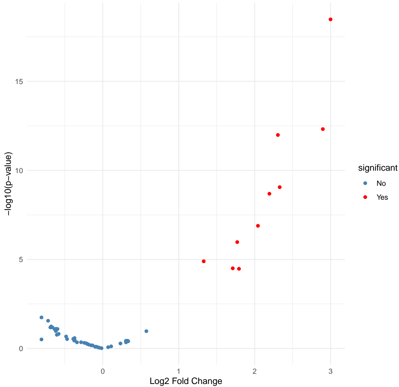
DESeq2 Volcano Plot
