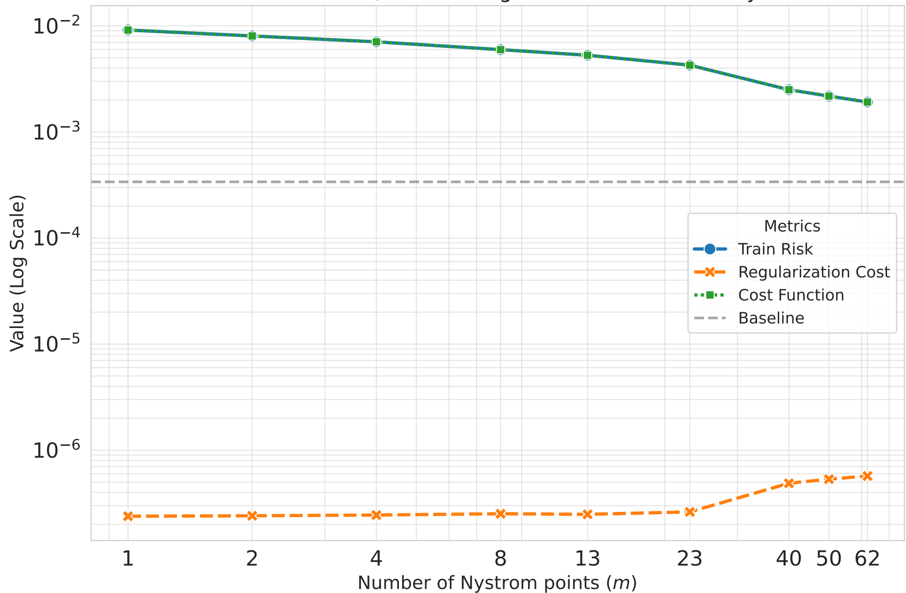
Cost function, risk and regularization terms decay
