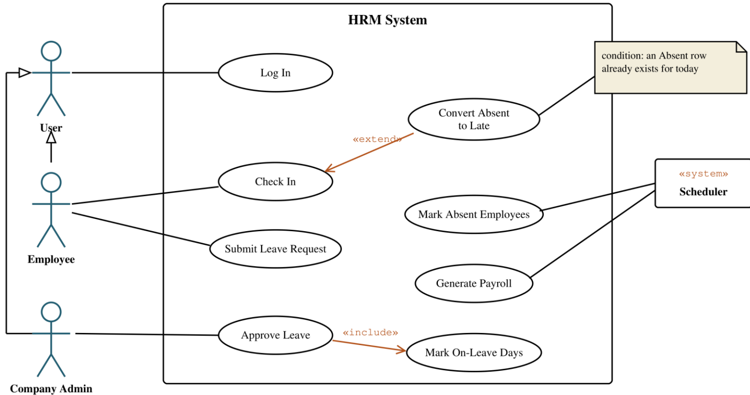
Figure: Use case diagram of the HRM System – Employee and Company Admin generalize User; Scheduler is a secondary «system» actor; Approve Leave «includes» Mark On-Leave Days; Convert Absent to Late «extends» Check In when an Absent row already exists.
