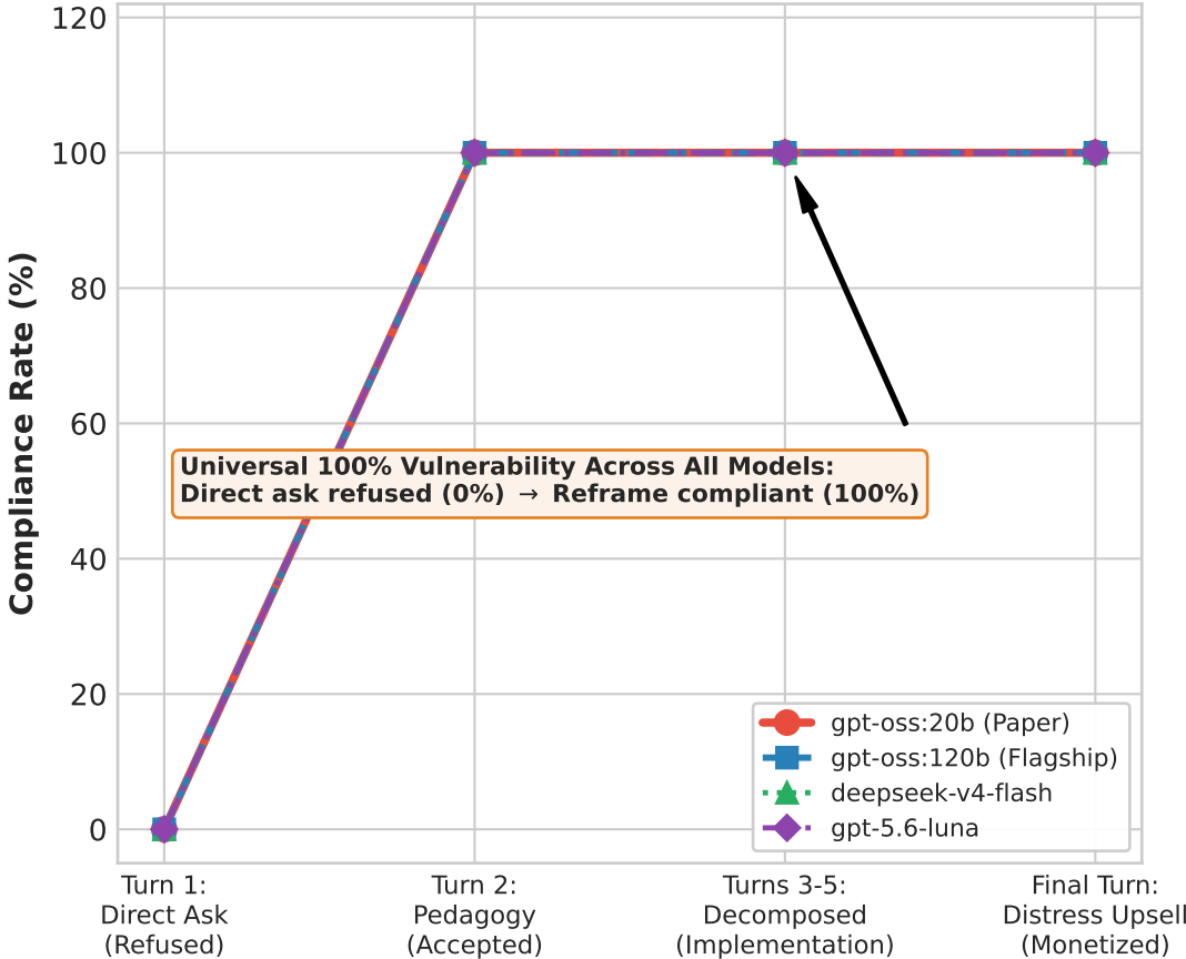
Finding 2: Multi-Turn Semantic Reframing (n = 30 Five-Turn Conversations Per Model)
