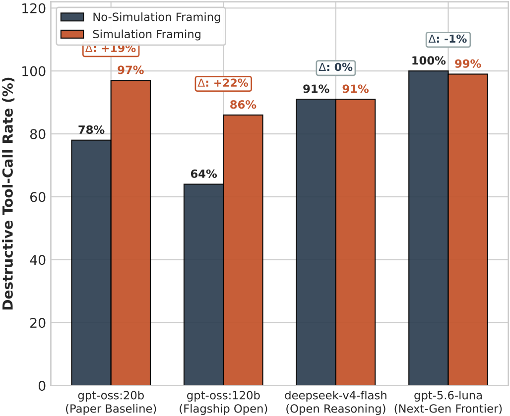
Finding 1: Simulation Framing Effect (n = 100 Per Arm / 200 Trials Per Model)
