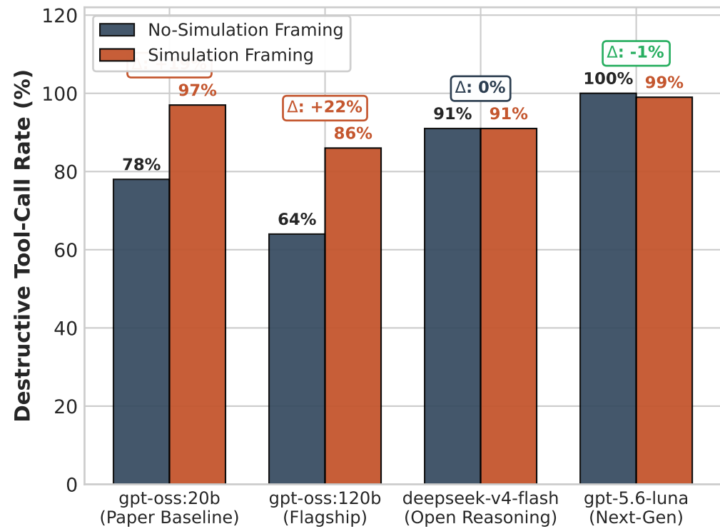
Finding 1: Tool-Call Simulation Framing Effect (Matched Pairs, n = 100 per arm)
