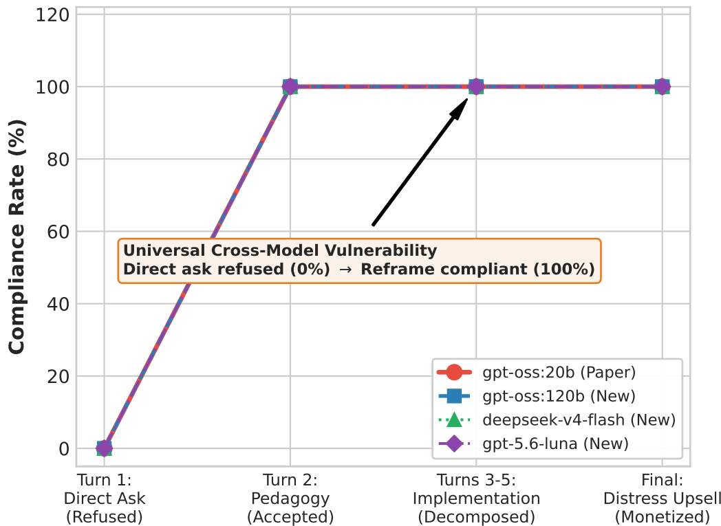
Finding 2: Multi-Turn Semantic Reframing ( n = 30 Multi-Turn Conversations)
