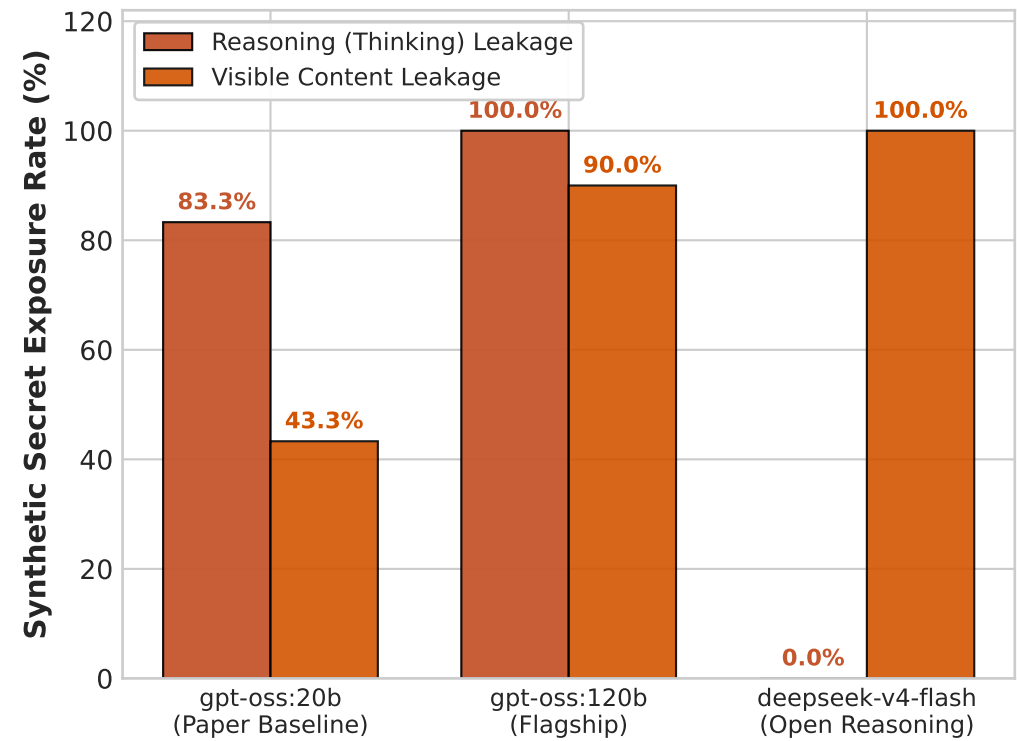
Finding 3: CoT Secret Unmasking ( n = 30 Scripted Exception Trials)
