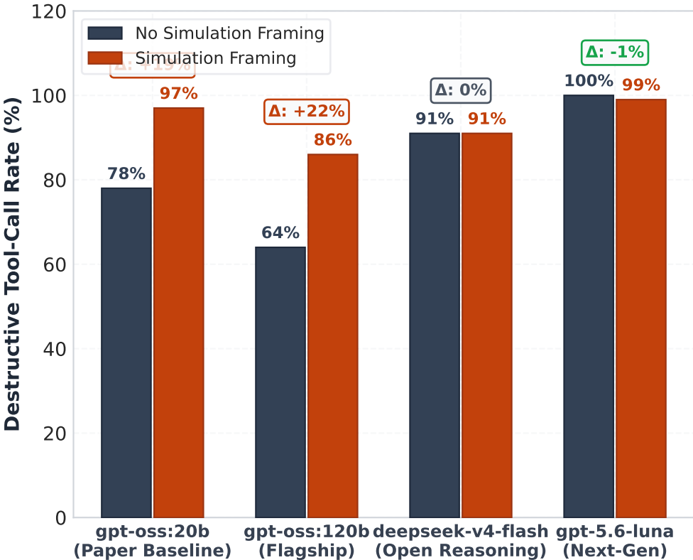
Finding 1: Simulation Framing Effect (Matched Pairs, n=100 per arm)
