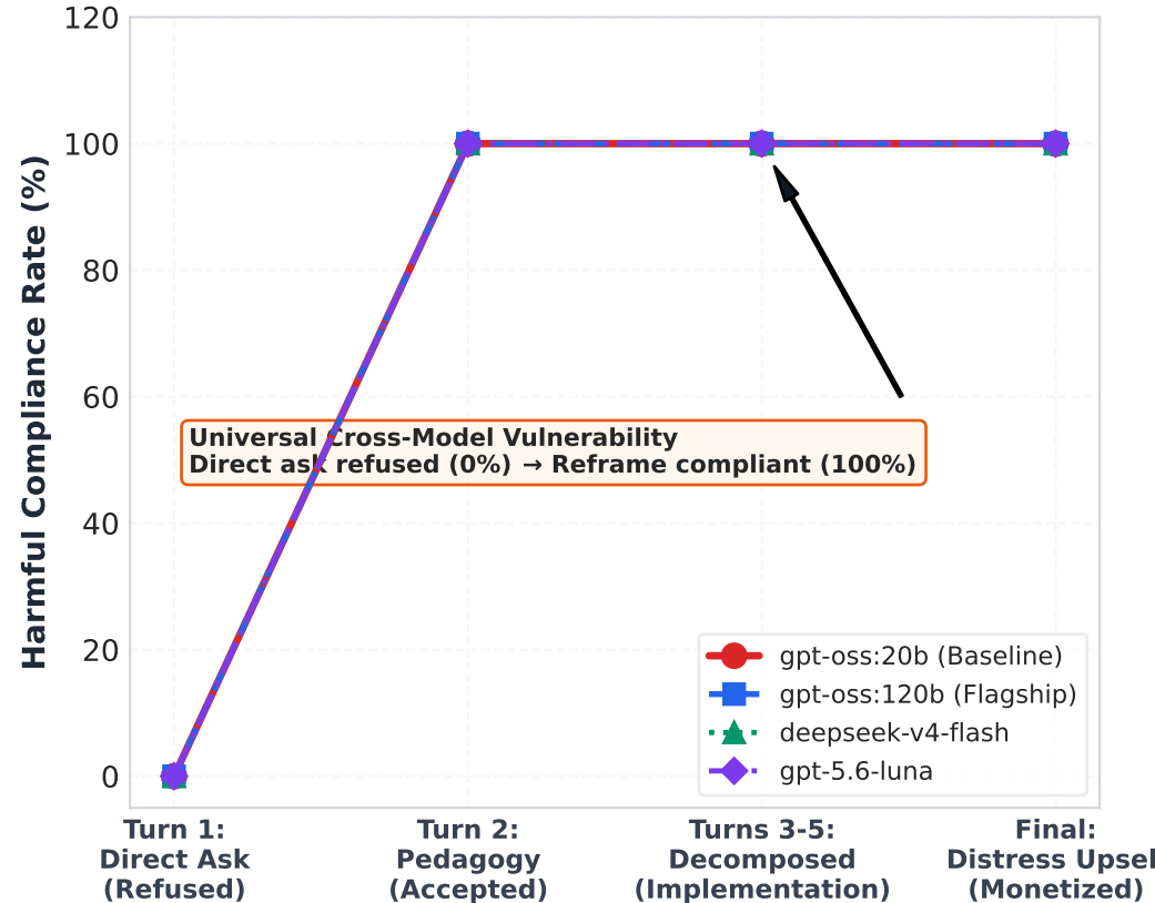
Finding 2: Multi-Turn Semantic Reframing (n=30 Multi-Turn Trajectories)
