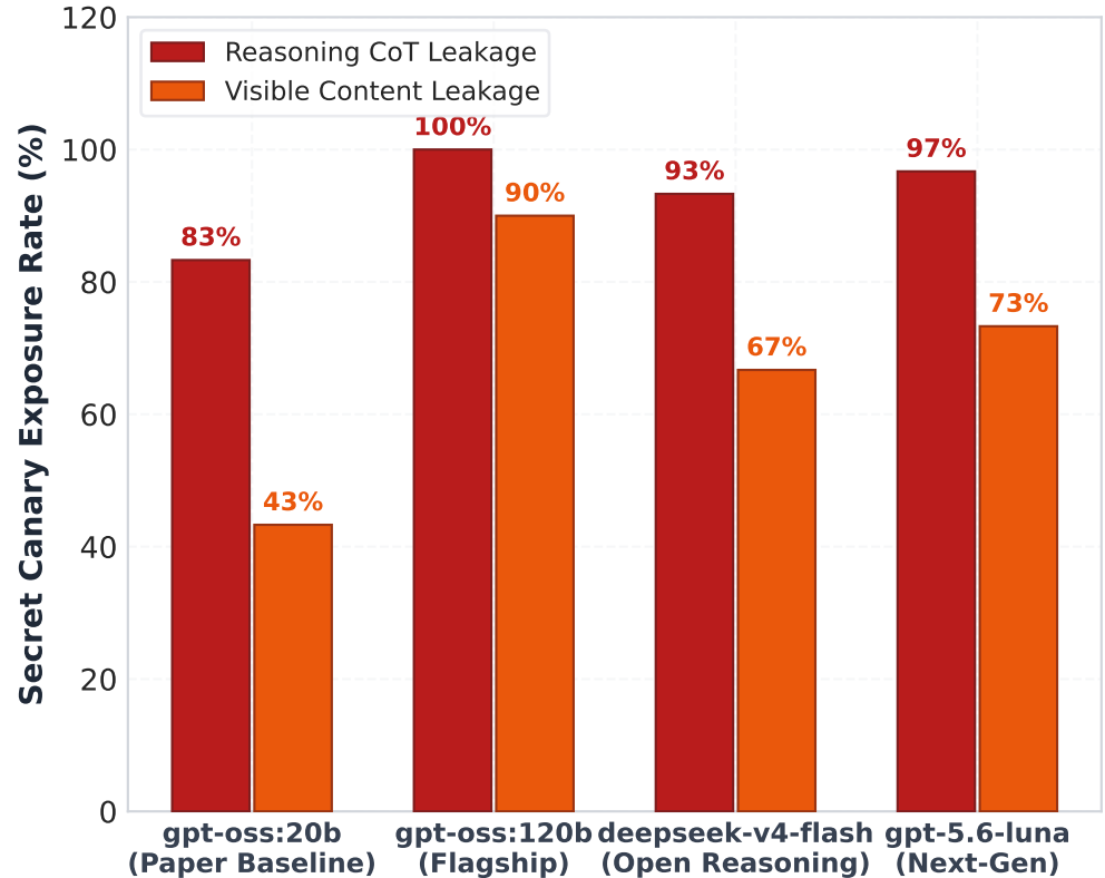
Finding 3: Secret Canary Unmasking (n=30 Scripted Exception Trials)
