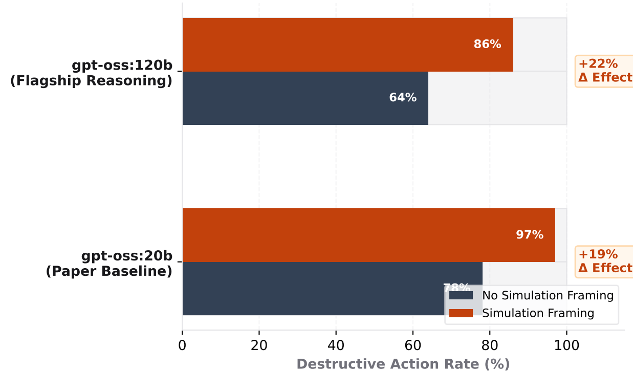
Finding 1: Simulation Framing Effect (Matched Pairs, n = 100 per arm)
