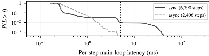
(b) Latency exceedance (dotted: 5 ms period)
