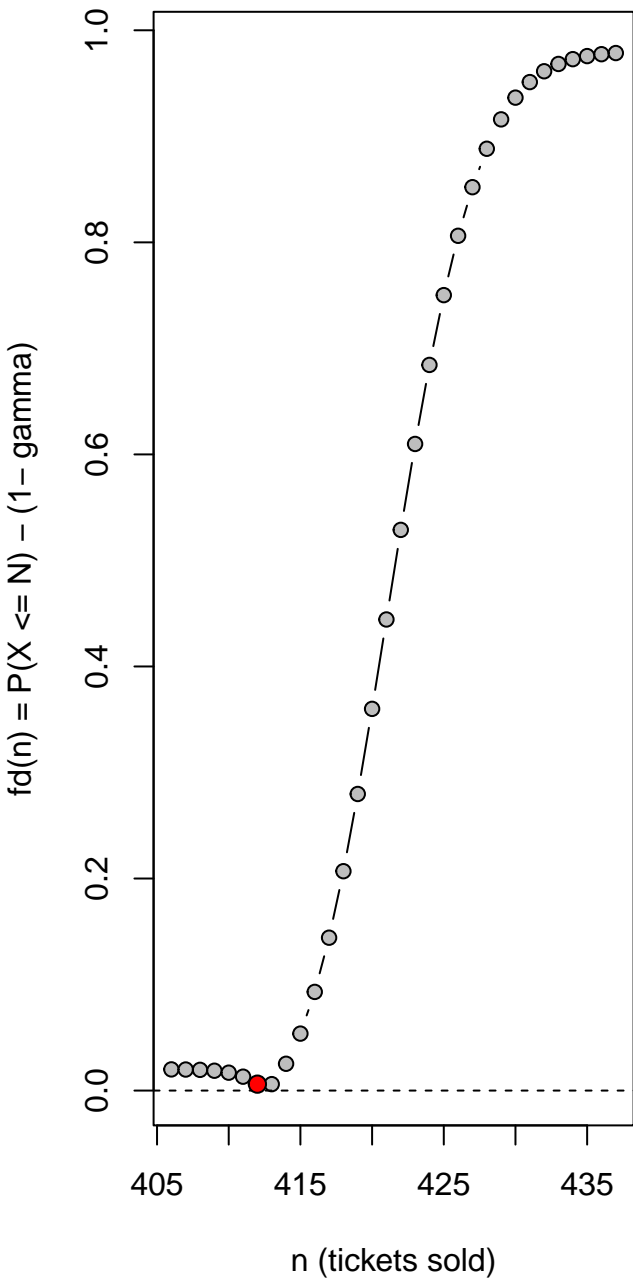
Discrete Objective
