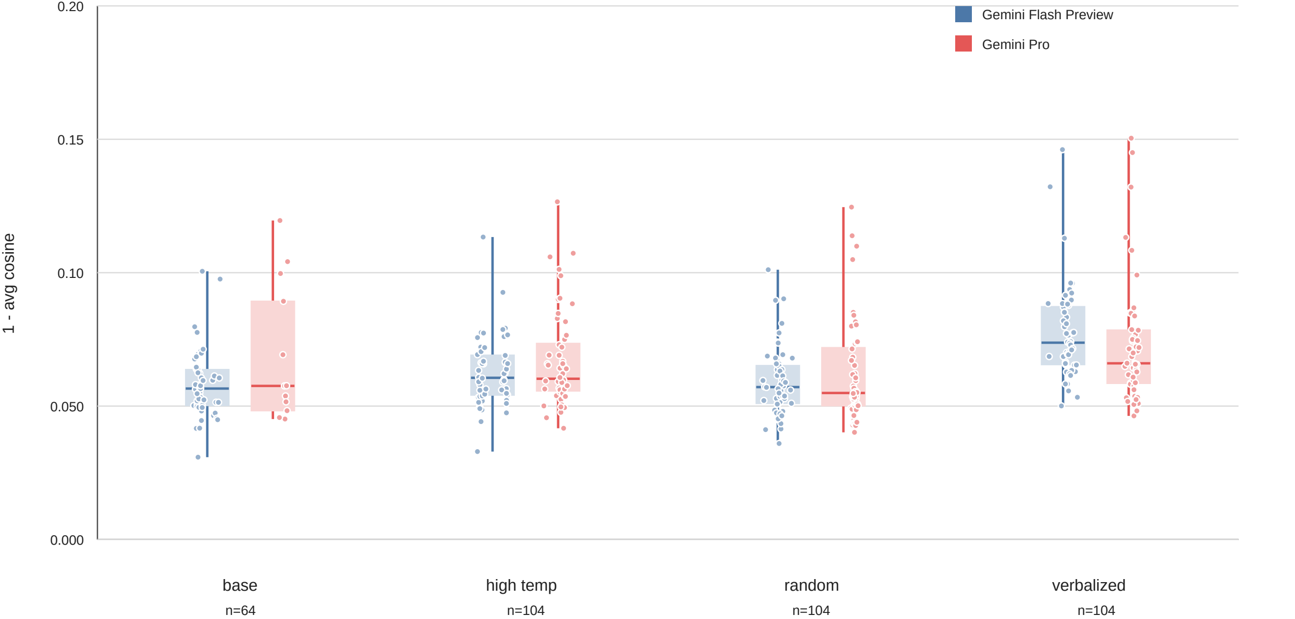
Trajectory diversity by model and method
