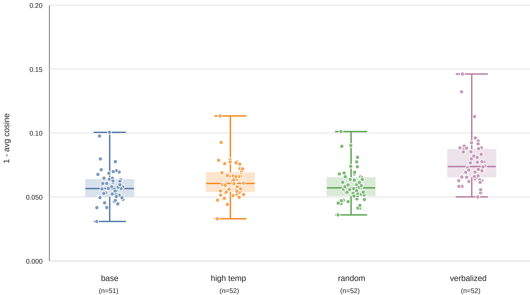
Trajectory diversity by sampling method
