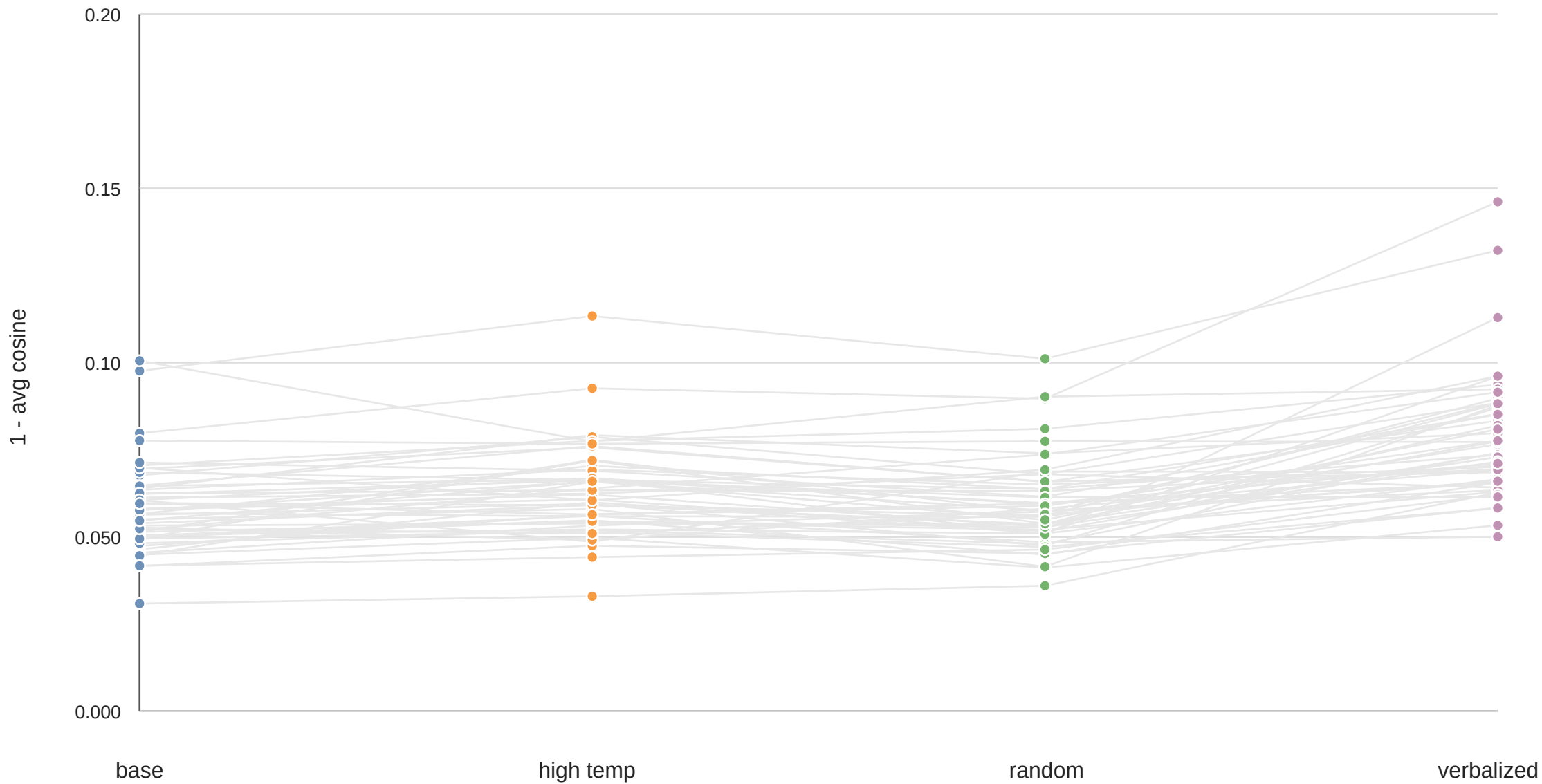
Paired task diversity by sampling method
