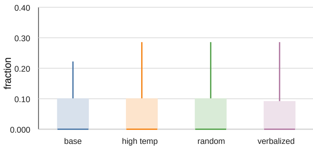
place_next_to
