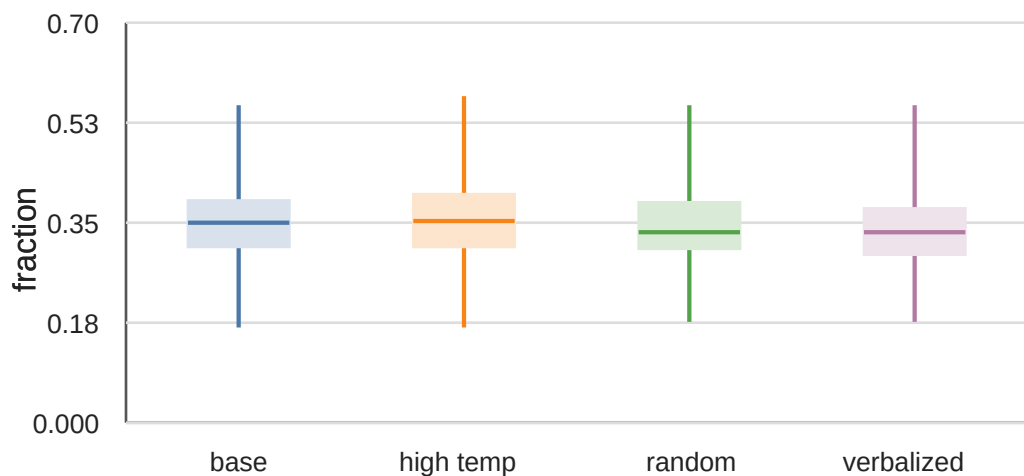
communicate
