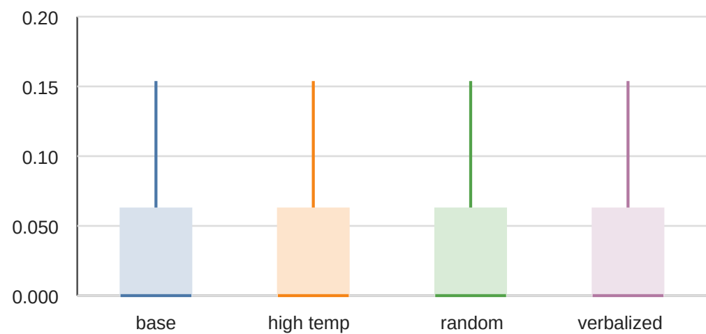
open_hinged_part
