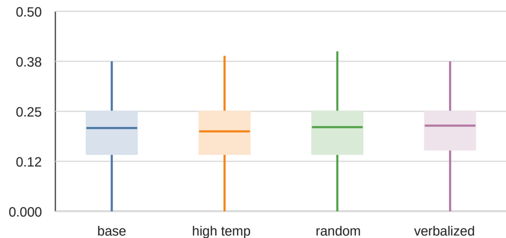
navigate_to_fixture
