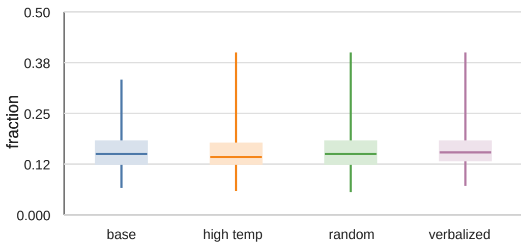
pick_up_object
