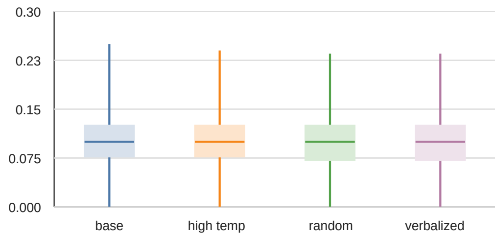
give_space
