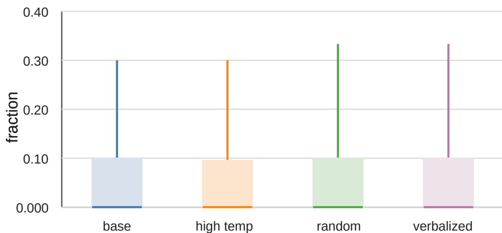
place_in_receptacle
