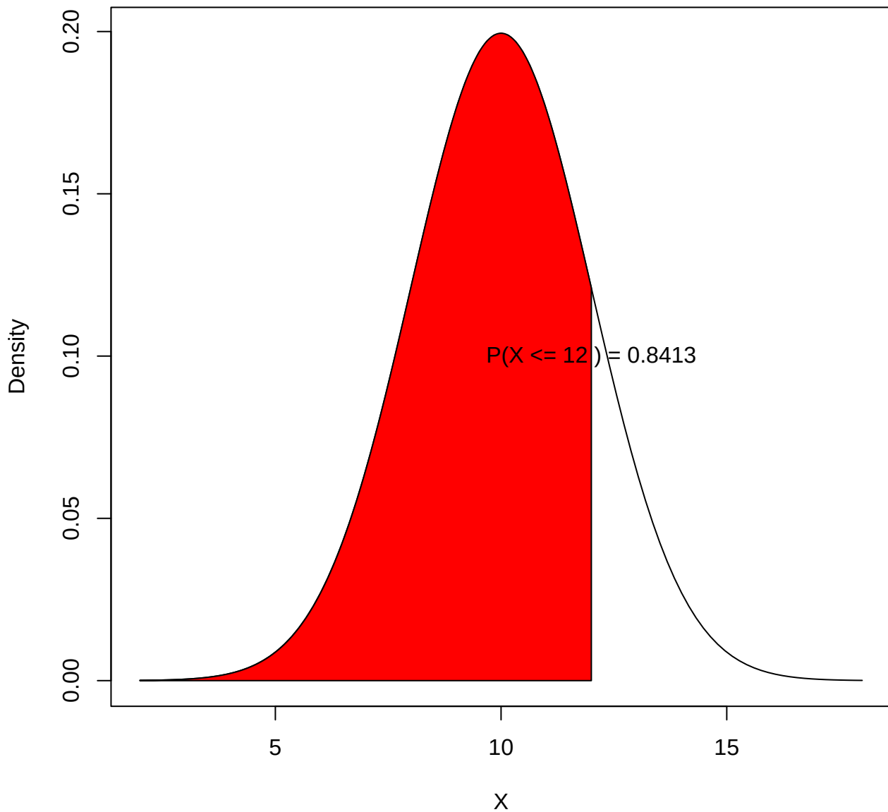
Normal Curve: mu = 10 , sigma = 2
