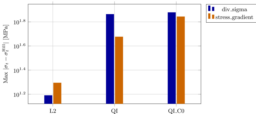
Max \sigma_t error vs Hill, max_level = 3
