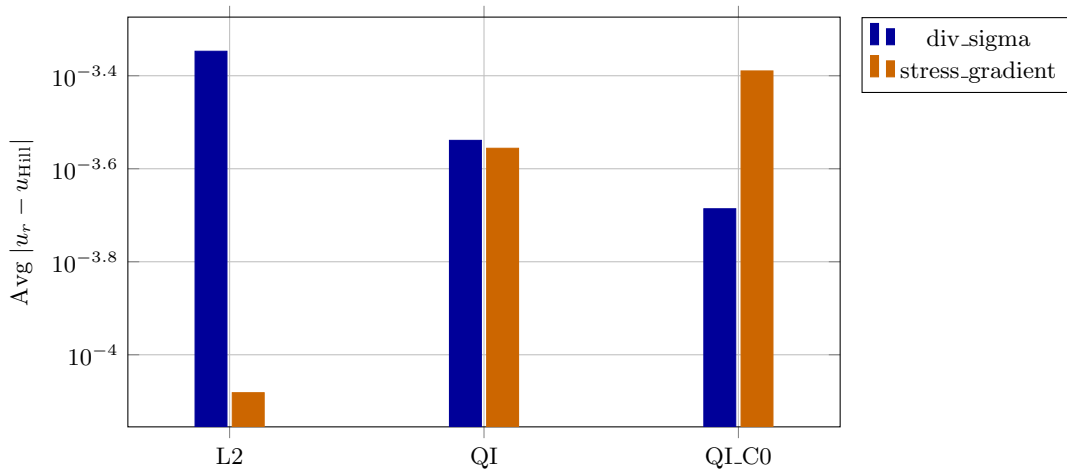
Avg u-error vs Hill, max_level = 3
