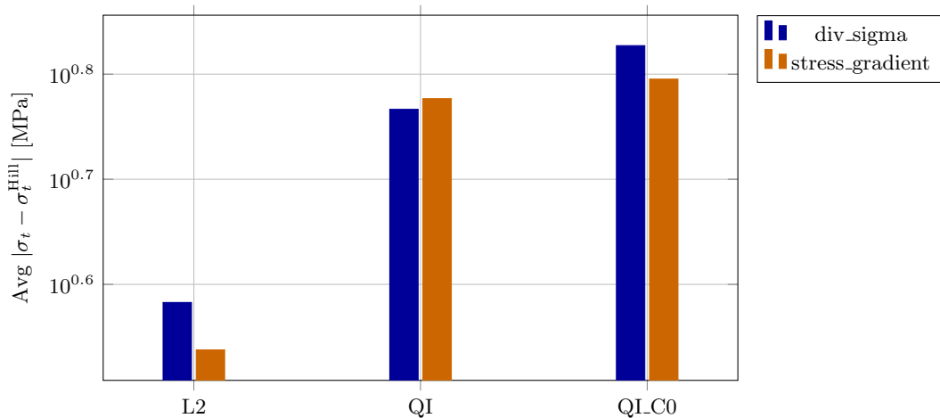
Avg \sigma_t error vs Hill, max_level = 3
