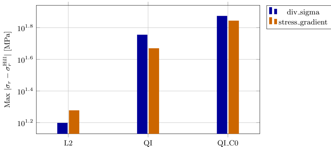
Max \sigma_r error vs Hill, max_level = 3
