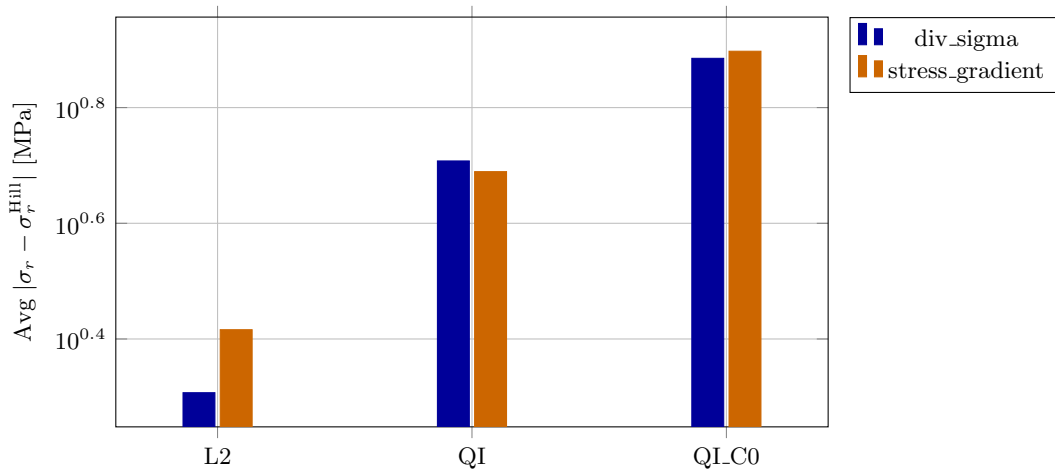
Avg \sigma_r error vs Hill, max_level = 3
