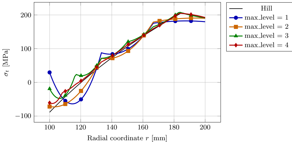
Tangential stress, QI C^0 , step 5
