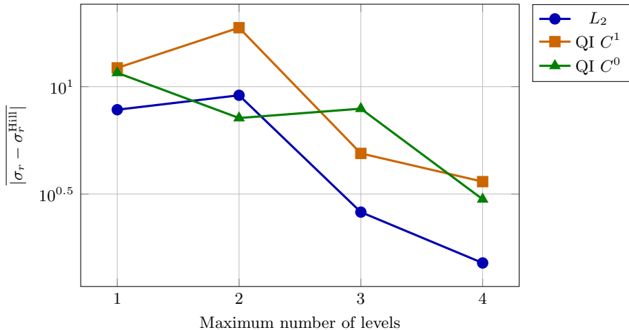
Avg \sigma_r error vs max_level
