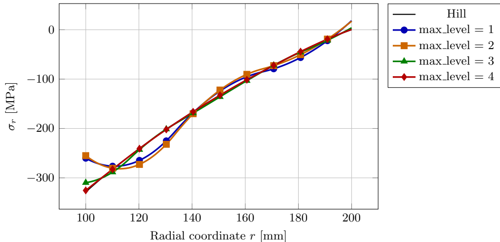
Radial stress, L_2 , step 5
