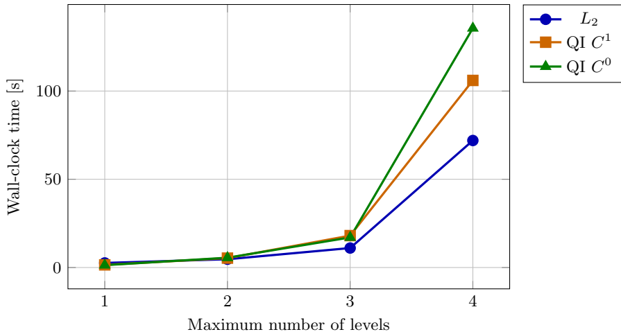
Cost vs max_level
