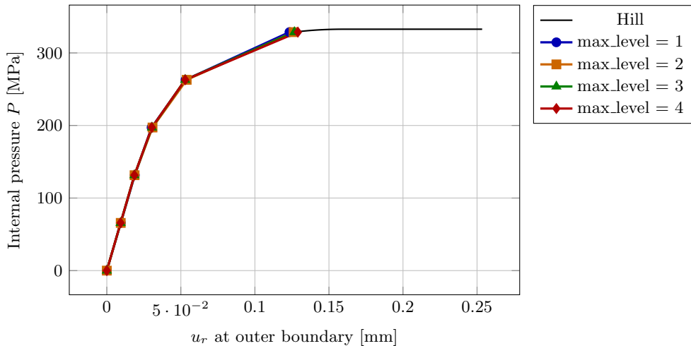
Load-displacement, L_2
