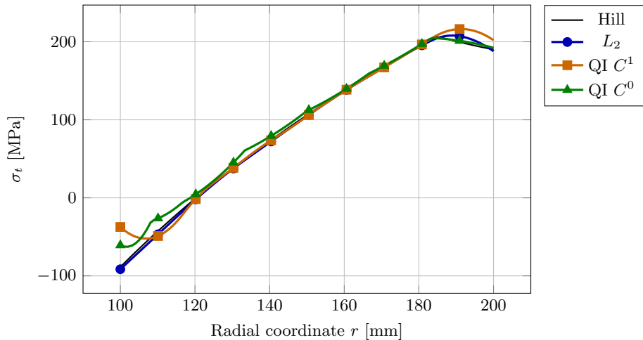
Tangential stress, step 5
