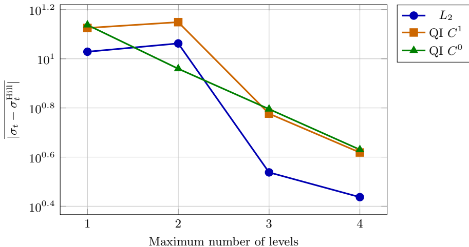
Avg \sigma_t error vs max_level
