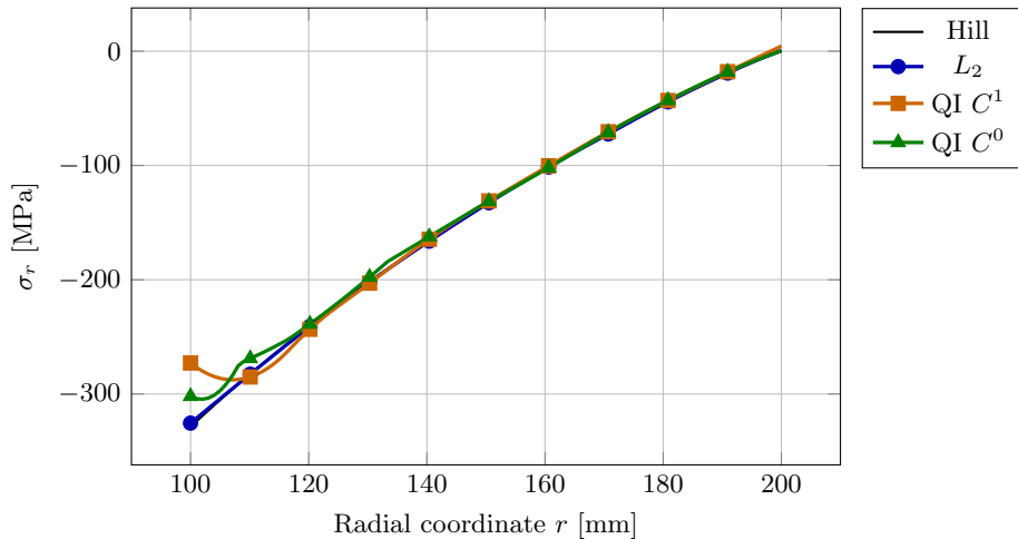
Radial stress, step 5
