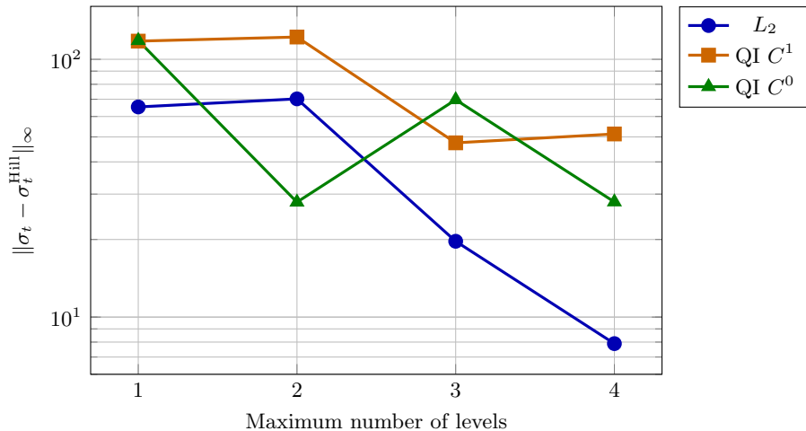
Max \sigma_t error vs max_level
