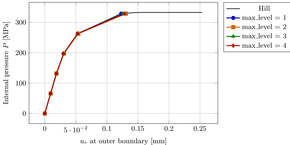
Load-displacement, QI C^0
