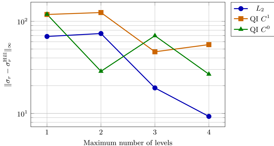
Max \sigma_r error vs max_level
