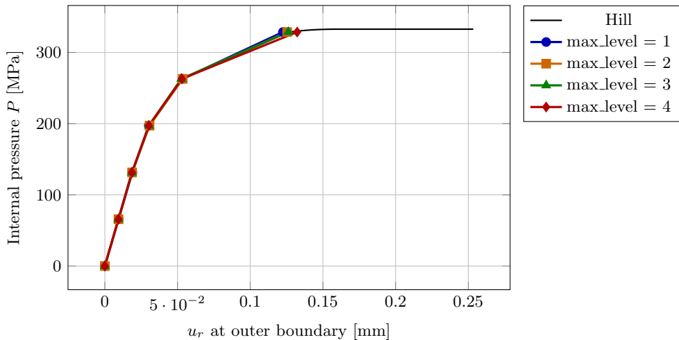
Load-displacement, QI C^1
