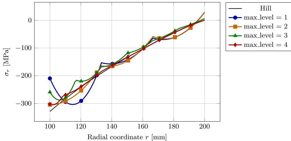
Radial stress, QI C^0 , step 5
