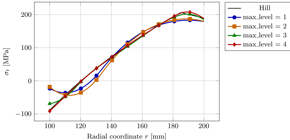
Tangential stress, L_2 , step 5
