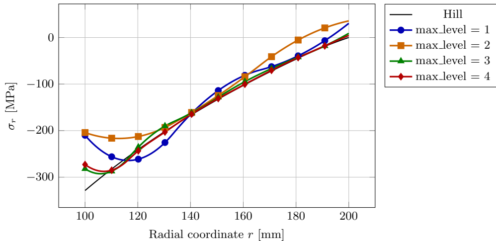
Radial stress, QI C^1 , step 5
