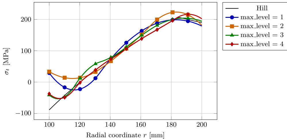
Tangential stress, QI C^1 , step 5
