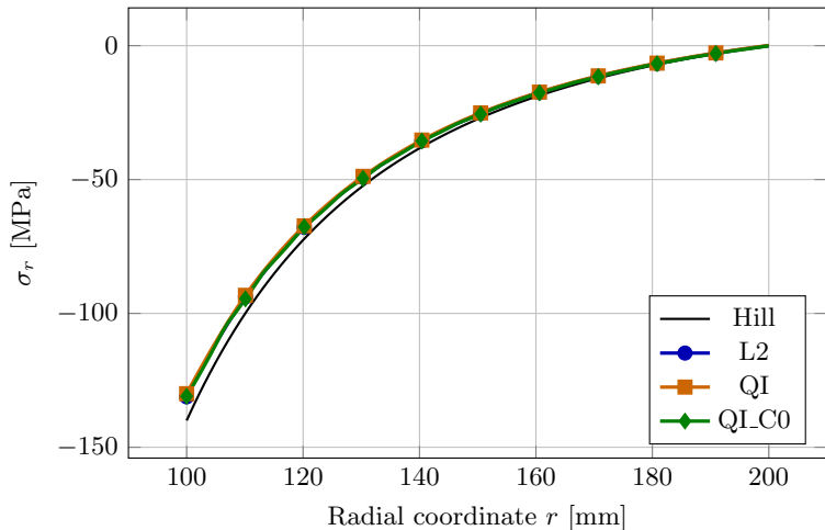
Radial stress, load step 2
