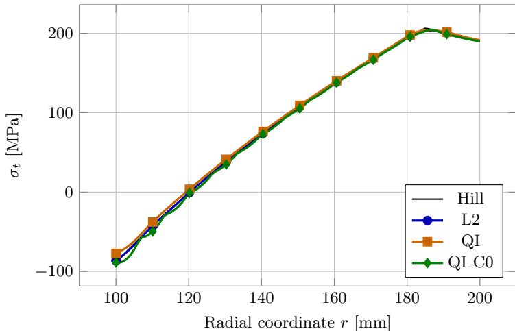
Tangential stress, load step 5
