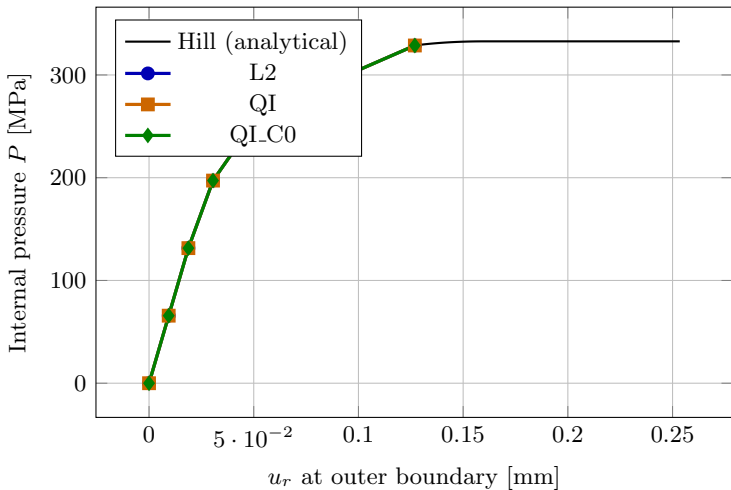
Eighth-sphere: load–displacement curve
