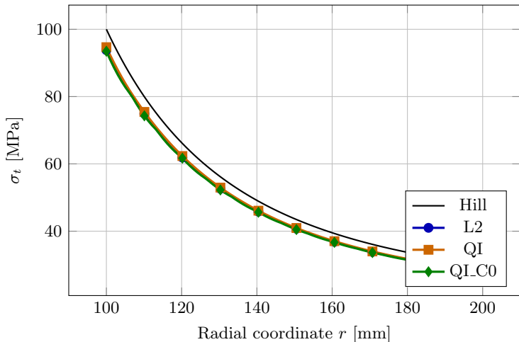
Tangential stress, load step 2
