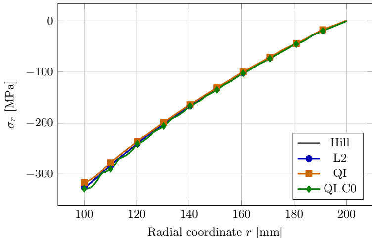
Radial stress, load step 5
