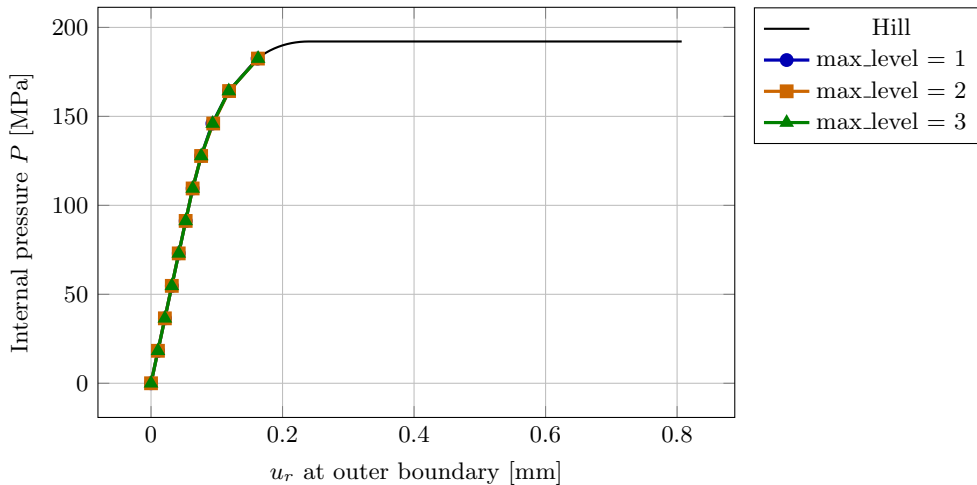
Load-displacement, QI C^1 (2D ring)
