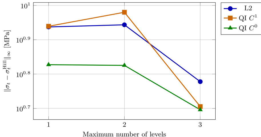
Max \sigma_t error vs max_level (2D ring)
