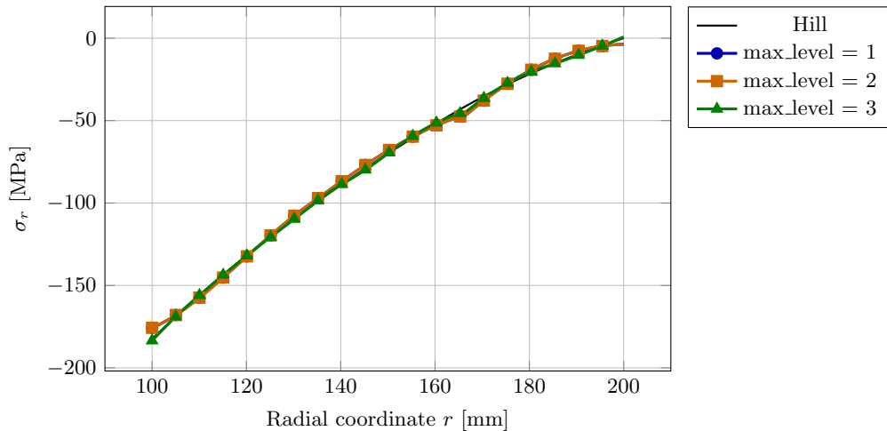
Radial stress, QI C^0 , step 10 (2D ring)
