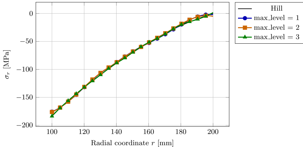
Radial stress, QI C^1 , step 10 (2D ring)
