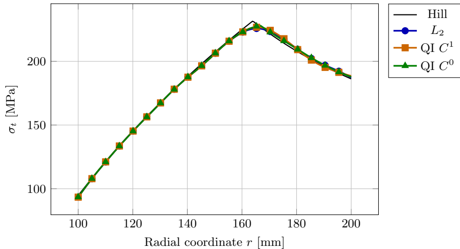
Tangential stress, step 10
