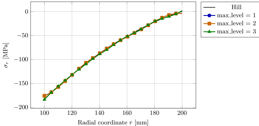
Radial stress, L2, step 10 (2D ring)
