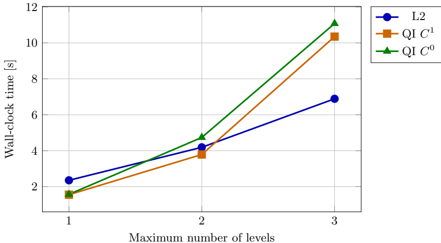
Cost vs max_level (2D ring)
