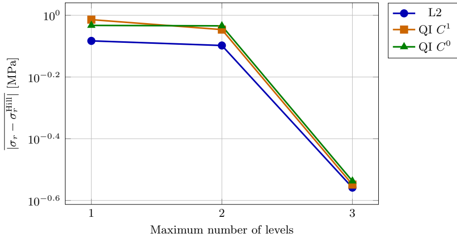
Avg \sigma_r error vs max_level (2D ring)
