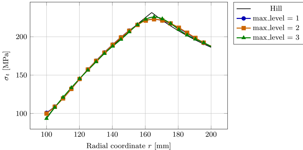
Tangential stress, L2, step 10 (2D ring)
