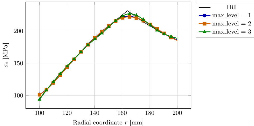
Tangential stress, QI C^1 , step 10 (2D ring)
