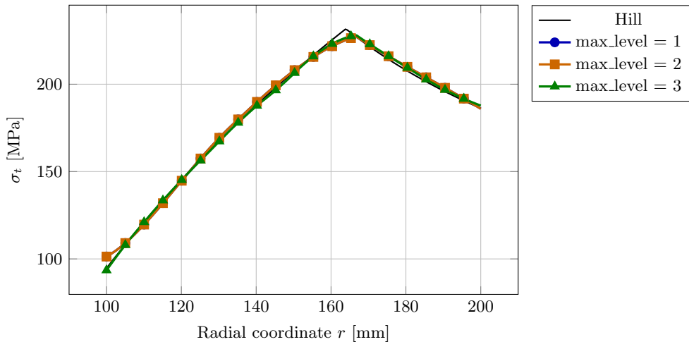
Tangential stress, QI C^0 , step 10 (2D ring)
