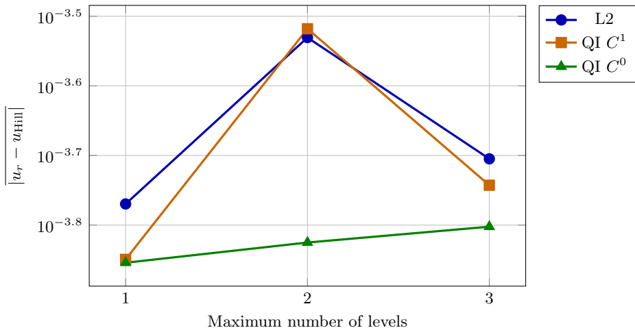
Avg u-error vs max_level (2D ring)
