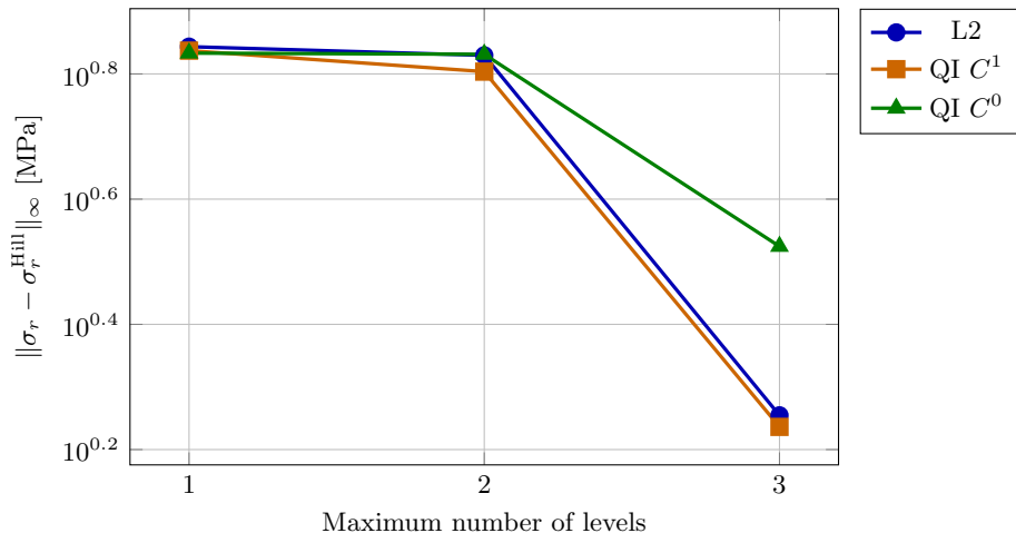
Max \sigma_r error vs max_level (2D ring)
