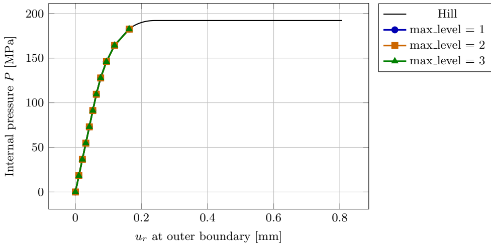
Load-displacement, L2 (2D ring)
