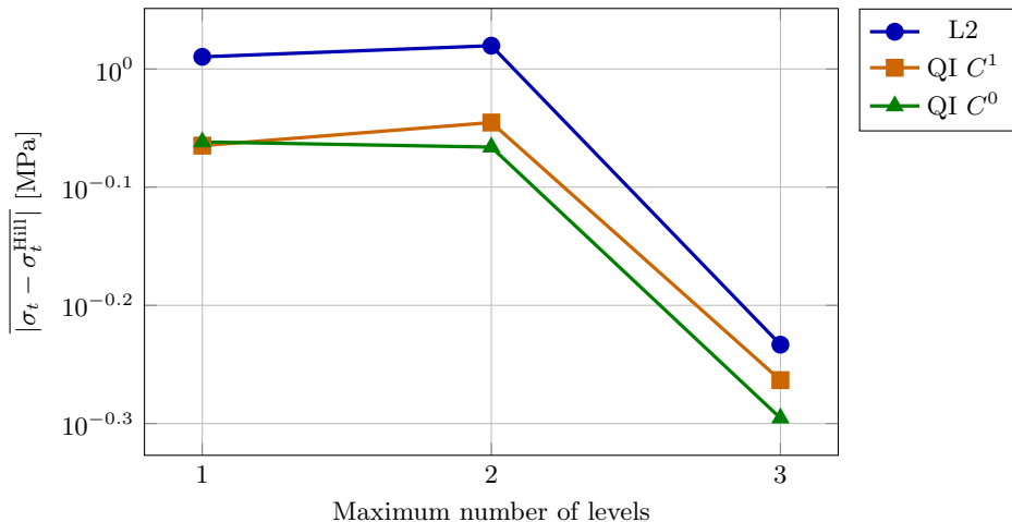
Avg \sigma_t error vs max_level (2D ring)
