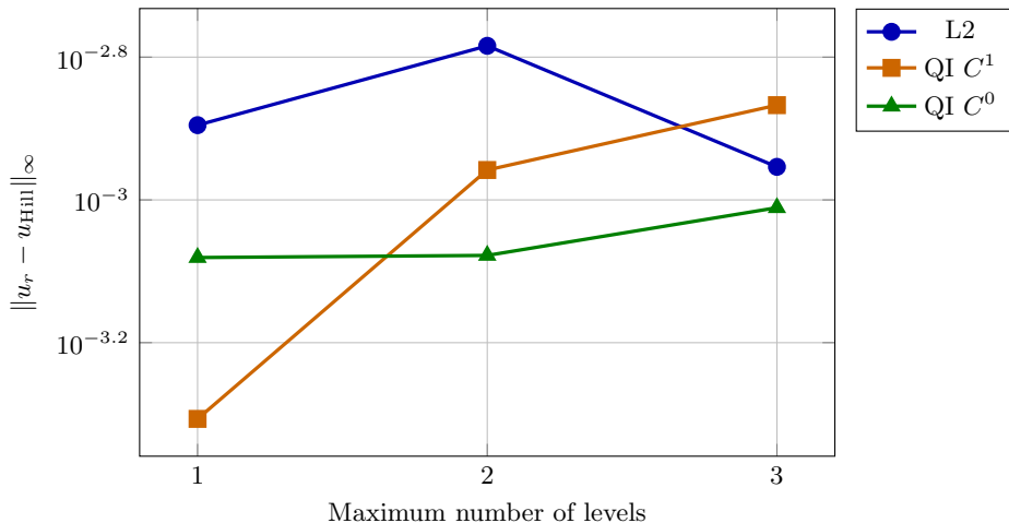
Max u-error vs max_level (2D ring)
