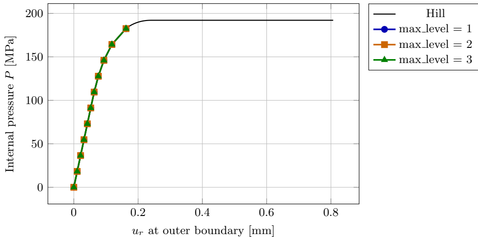
Load-displacement, QI C^0 (2D ring)
