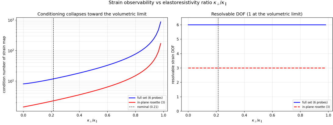
Figure 6: Strain observability vs the elastoresistivity ratio \kappa_{\perp}/\kappa_{\parallel} . Left: condition number of the strain map for an in-plane rosette and a full set, diverging as the response becomes volumetric. Right: resolvable DOF, full for any anisotropic response. The dashed line marks the thesis-anchored ratio ( \approx 0.21 ).
