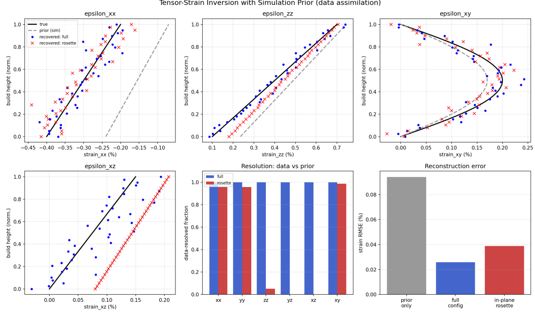
Figure 7: Tensor-strain inversion with a biased simulation prior. In-plane components ( \epsilon_{xx}, \epsilon_{xy} ) are corrected from data by both configurations; out-of-plane components ( \epsilon_{zz}, \epsilon_{xz} ) are recovered only by the full set and otherwise follow the prior, consistent with the resolution diagonal (centre).
