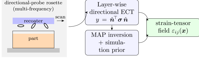
Figure 1: Proposed deployment. A recoater-mounted, multi-frequency directional-probe rosette scans each layer; the directional measurements are fused with a thermomechanical process-simulation prior by a regularised (MAP) inversion to reconstruct the strain-tensor field. This schematic doubles as the graphical abstract.
