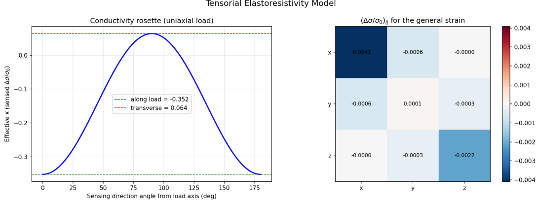
Figure 3: Tensorial elastoresistivity. Left: the “conductivity rosette” — the effective \kappa sensed in a uniaxial test depends on the sensing angle, swinging from -0.35 (along load) to +0.06 (transverse). Right: the induced (\Delta\sigma/\sigma_0)_{ij} tensor for the strain \varepsilon_{xx} = 1.0\% , \varepsilon_{yy} = -0.3\% , \varepsilon_{zz} = 0.4\% , \varepsilon_{xy} = 0.2\% , \varepsilon_{yz} = 0.1\% (illustrative \kappa_{\parallel} = -0.40 , \kappa_{\perp} = -0.08 ).
