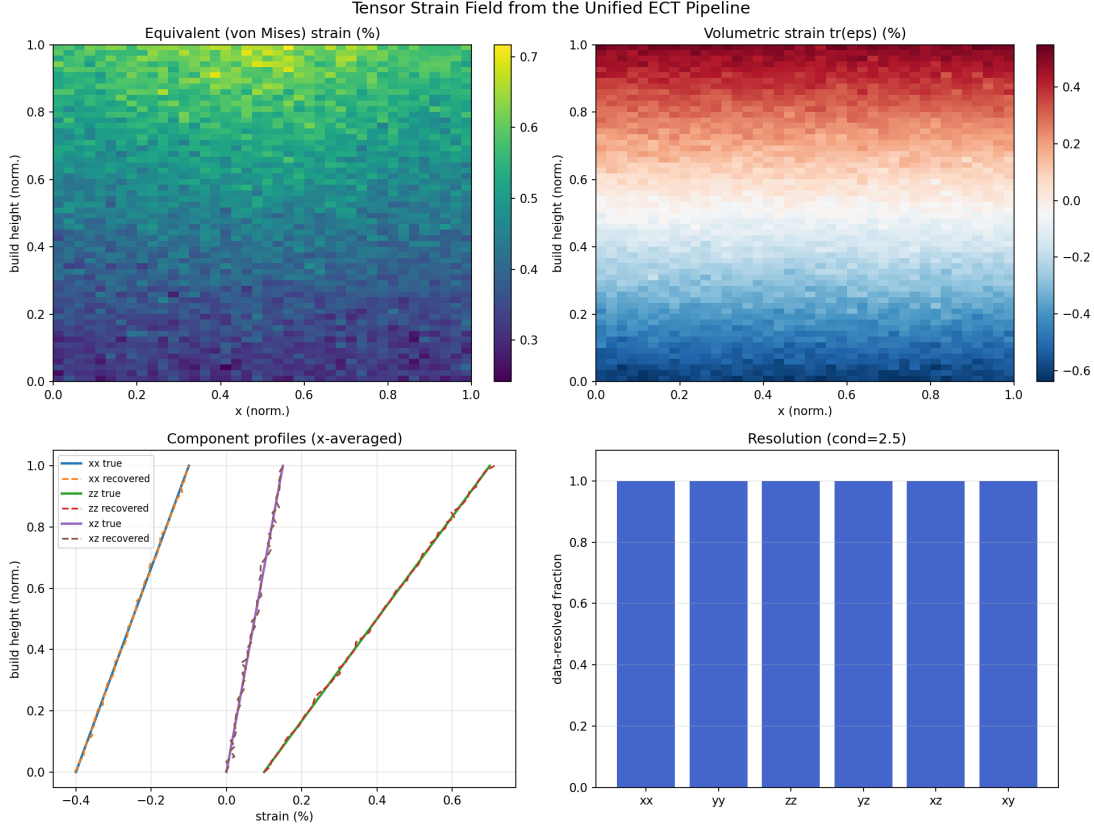
Figure 8: Strain-tensor field reconstructed by the unified pipeline. Equivalent (von Mises) and volumetric strain fields over the build (top), component profiles versus build height (bottom-left) and the per-component data resolution (bottom-right).
