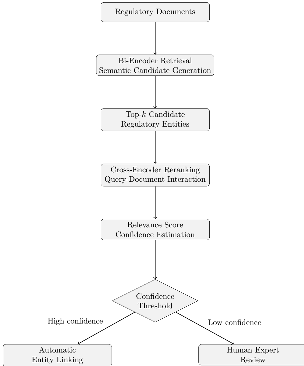
Figure 3.1: Conceptual overview of the proposed regulatory document entity linking framework.
