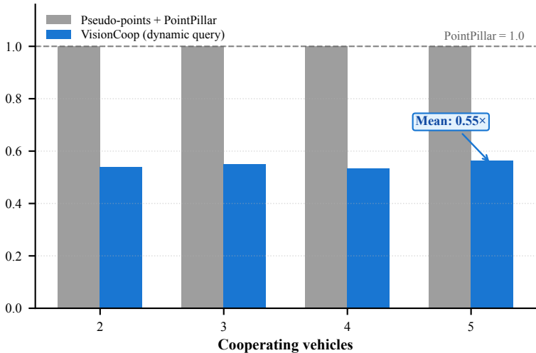
Relative inference cost (PointPillar = 1.0)
