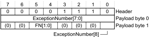
Figure D-15 Exception trace packet format
