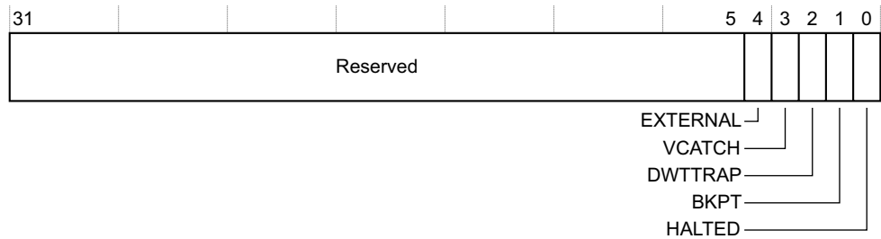
Figure C1-2 DFSR bit assignments
