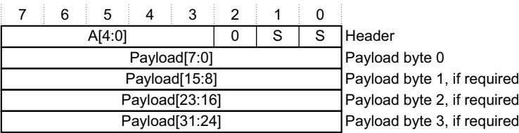
Figure D-11 Instrumentation packet format
