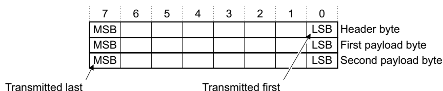
Figure D-1 Convention for packet descriptions
