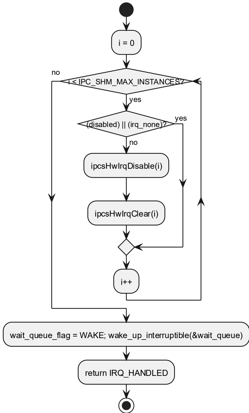
6.7.12 ipcsShmHardirq processing flow
