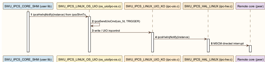
Linux UIO transmit notify sequence
