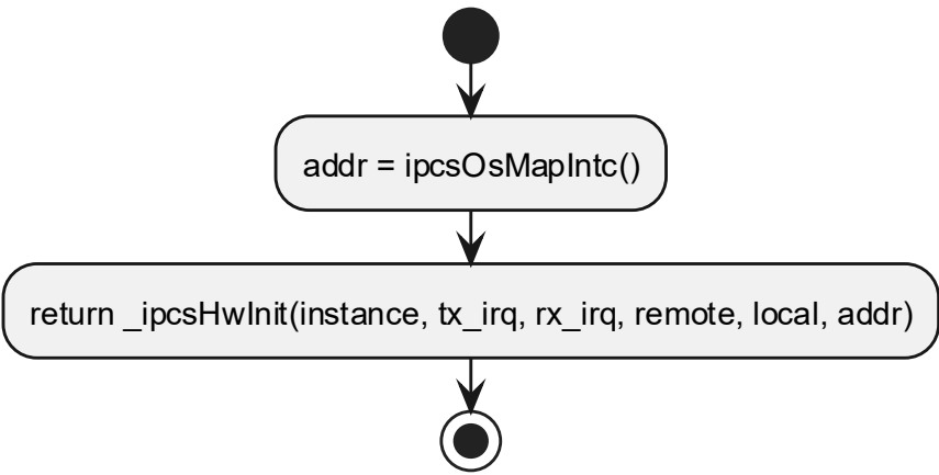
6.8.2 ipcsHwInit processing flow
