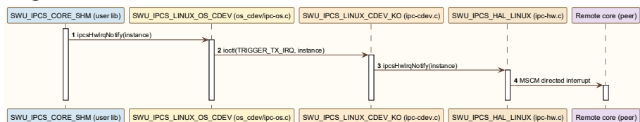
Linux CDEV transmit notify sequence
