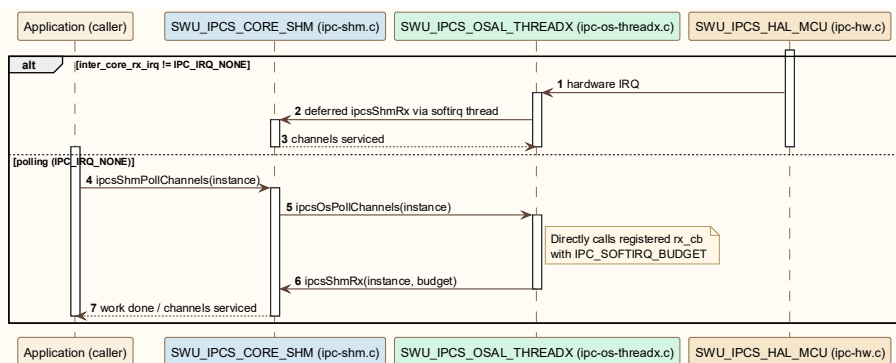
RTOS IRQ and polling sequence
