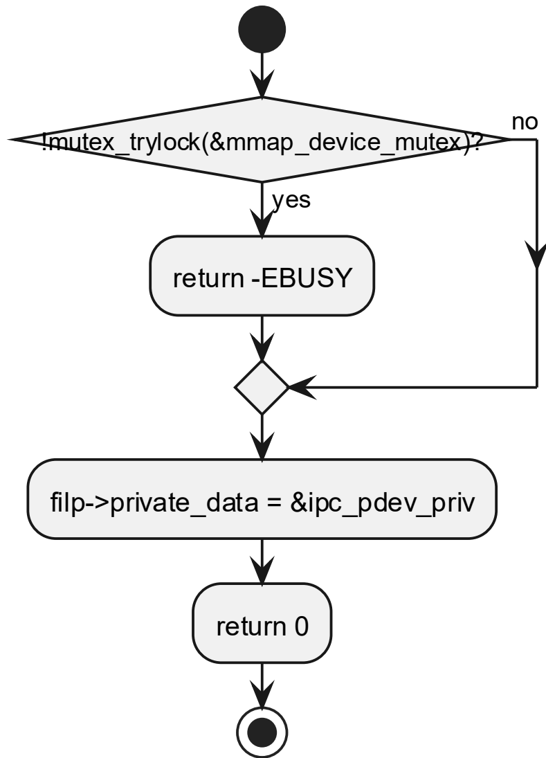
6.5.22 ipcsCdevOpen processing flow
