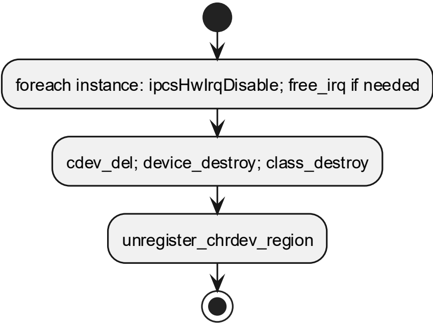
6.7.21 ipcsCdevClean processing flow
