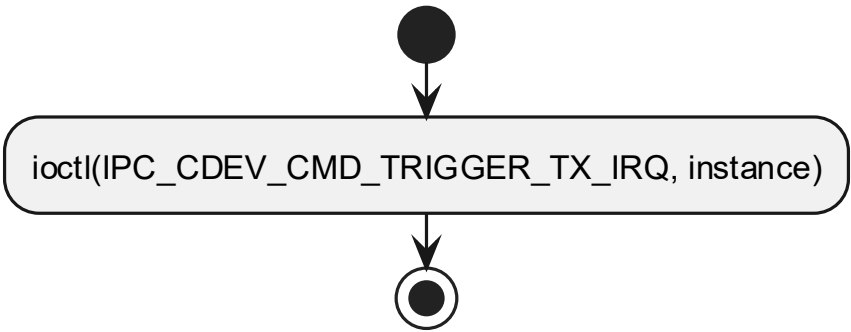
6.6.8 ipcsHwIrqNotify processing flow
