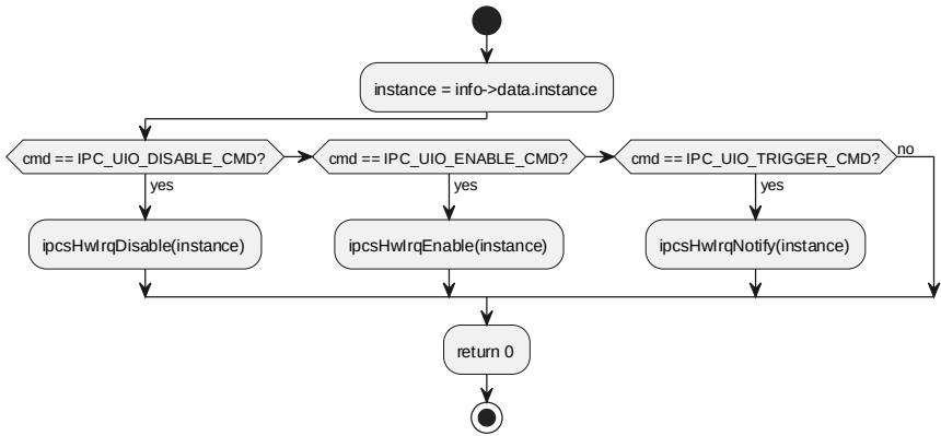
6.5.19 ipcsShmUioIrqcontrol processing flow
