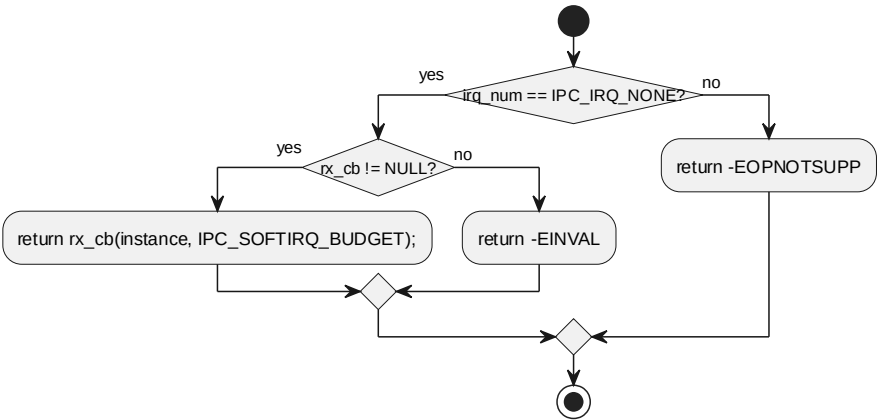
6.3.9 ipcsOsPollChannels processing flow
