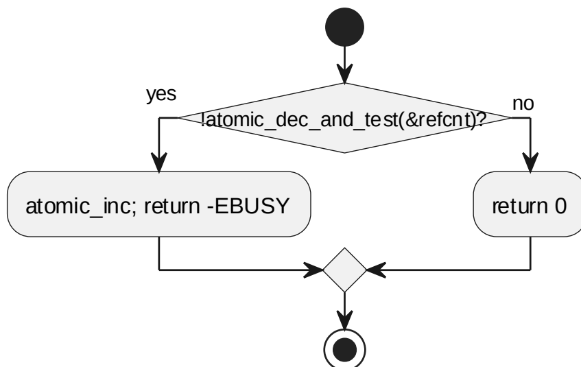
6.5.17 ipcsShmUioOpen processing flow
