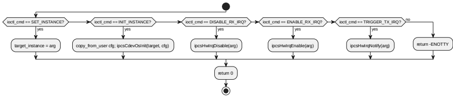
6.7.19 ipcsCdevIoctl processing flow
