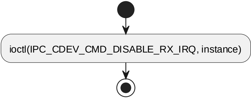
6.6.7 ipcsHwIrqDisable processing flow
