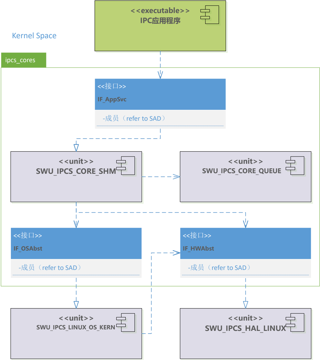
Linux in-kernel interface and SWU relationship
