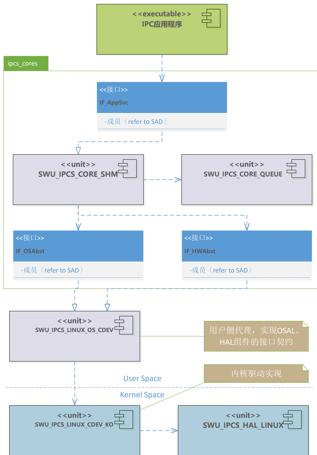
Linux CDEV interface and SWU relationship
