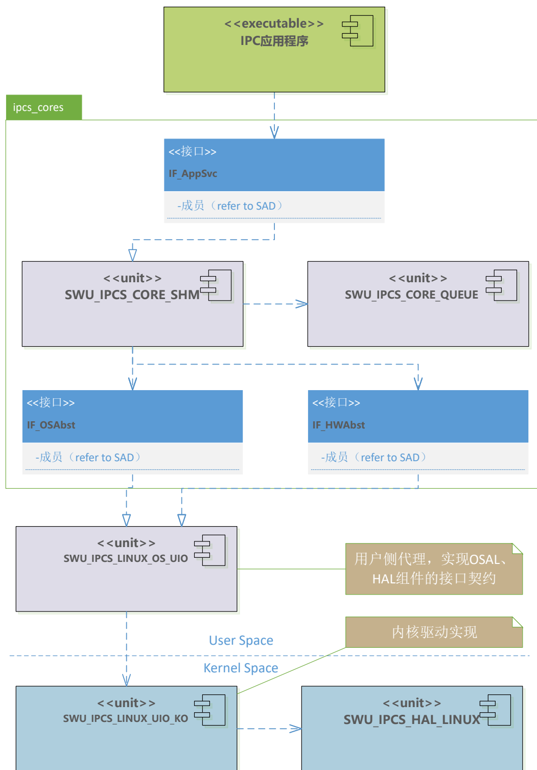
Linux UIO interface and SWU relationship
