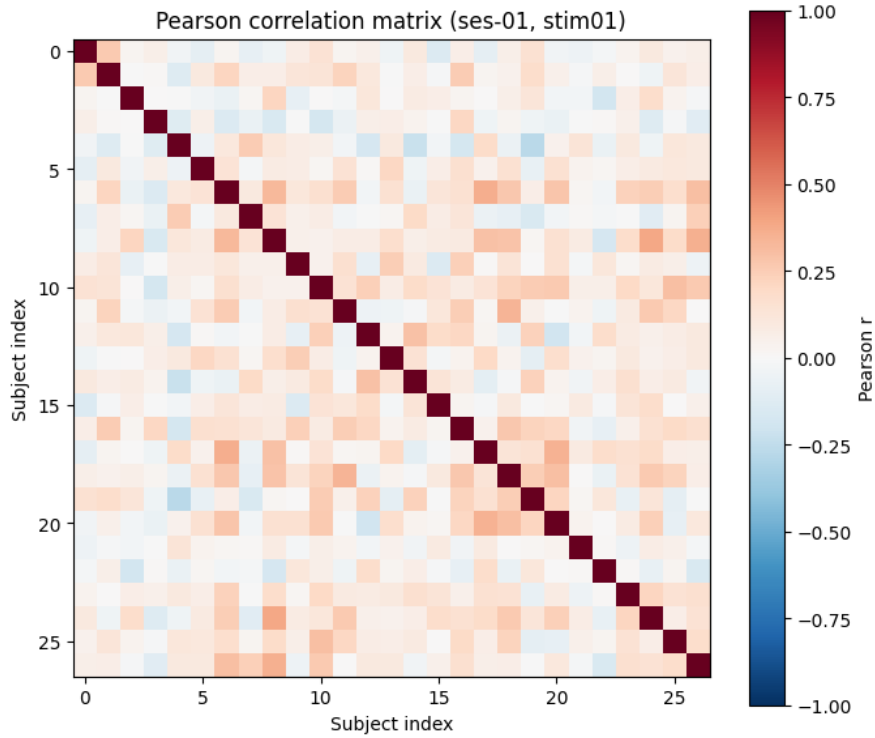
Fig. 4 Pearson correlation matrix. Entry (i, j) is the Pearson correlation between subject i and subject j . The dark diagonal is each subject with itself ( r = 1 )
