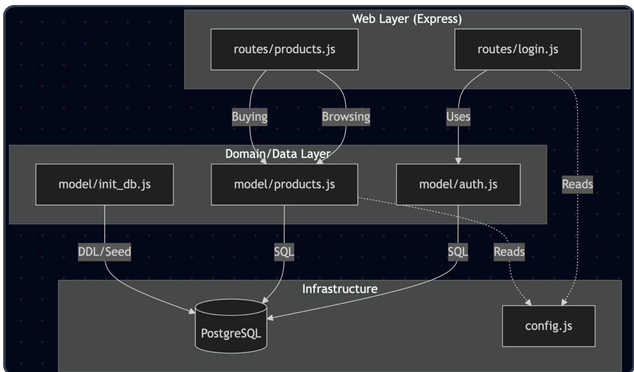
Figure 1: Architecture Diagram — Context Map Visualization
