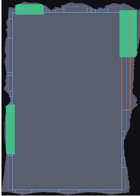
Figure 1: The certificate of segment 20230702185753, as vesuve grand-prize writes it: 6333 of 97771 chunks certified. Green: certified chunks; grey: present and not certified. Outlines: blue, the loops whose seams it would still have to measure; orange, a loop whose closure crosses half a sheet.
