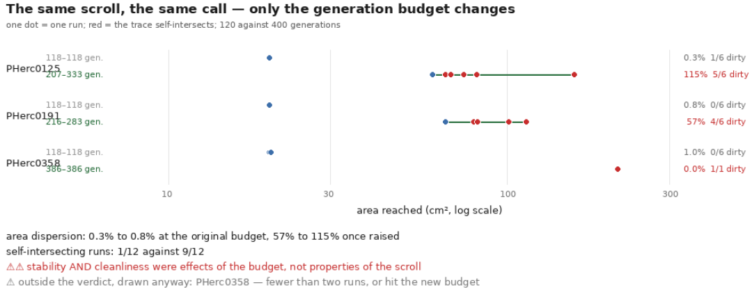
Figure 7: The same scroll, the same call, six runs each; only the generation budget changes (120 against 400). One dot per run, red if the trace self-intersects. The upper row of each pair is the original budget — six runs collapsed onto one point — and the lower row is the raised budget.
