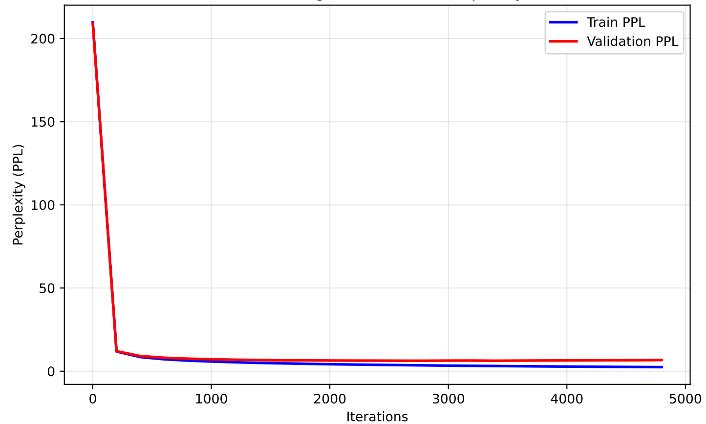
SFT Training and Validation Perplexity
