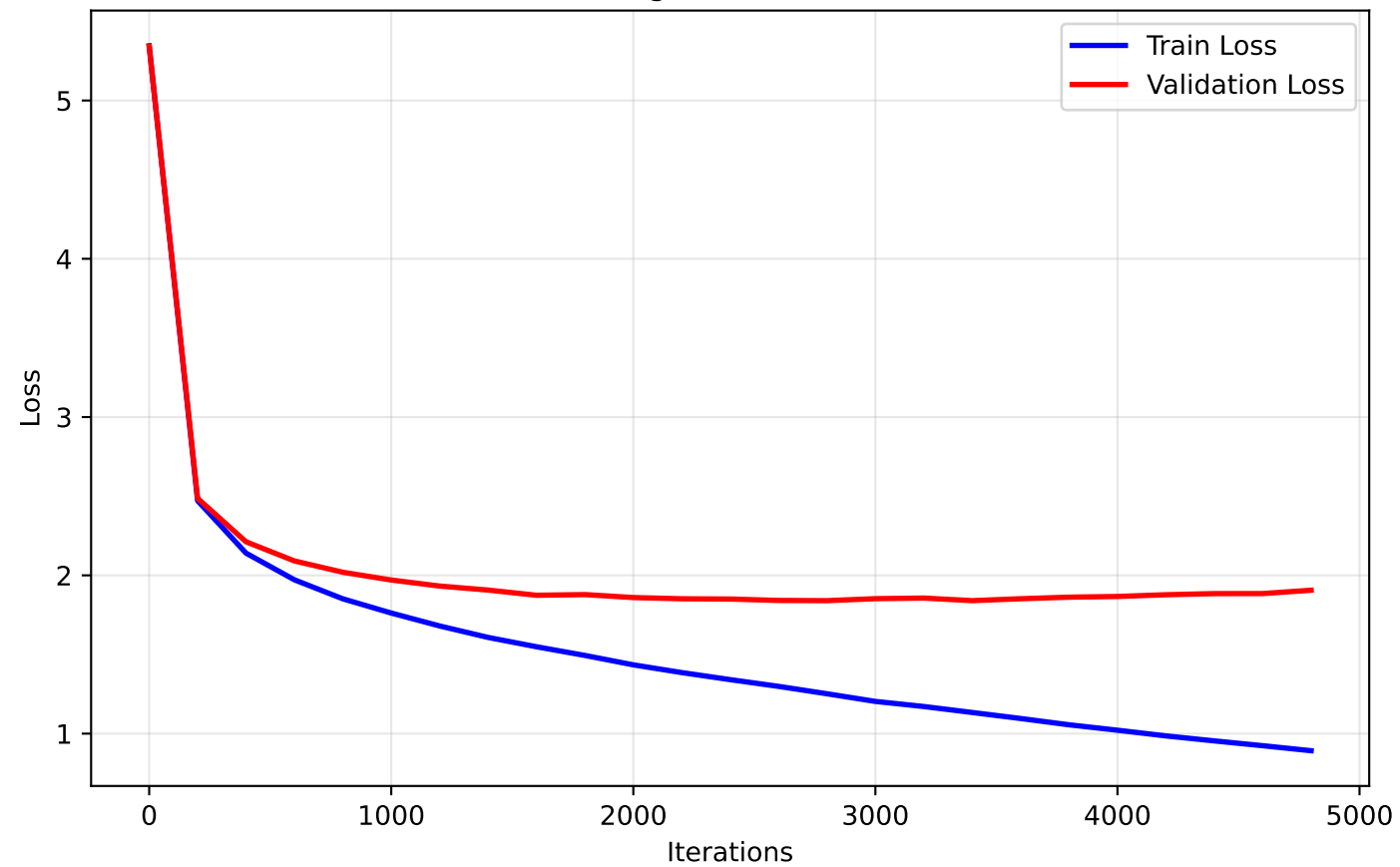
SFT Training and Validation Loss
