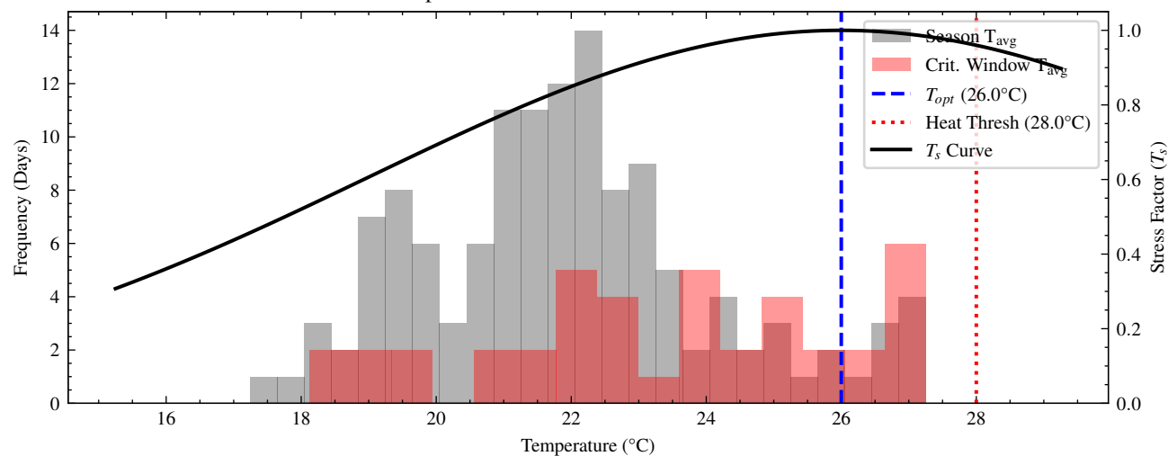
Temperature Distribution &amp; Gaussian Stress
