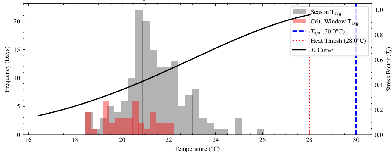
Temperature Distribution & Gaussian Stress
