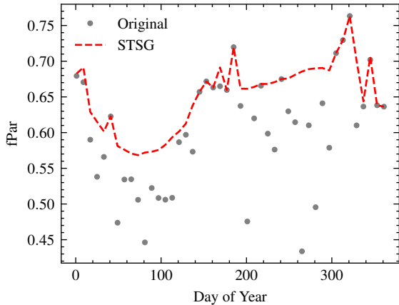
fPar (2020)
