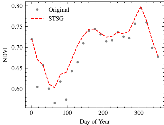
NDVI (2020)
