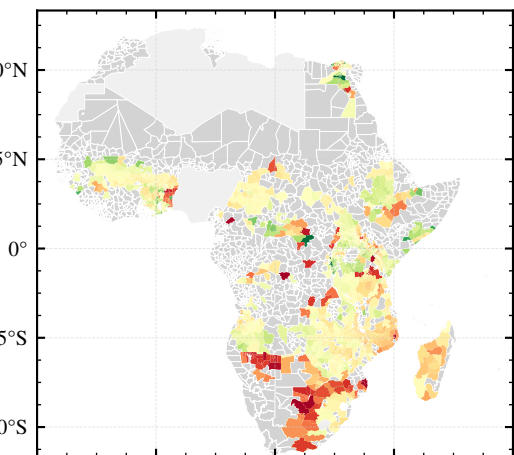
2015 Detrended Yield Anomaly
