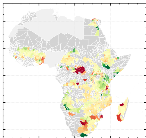
2020 Detrended Yield Anomaly
