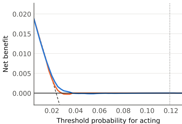
D Decision curve, shoulder IL
