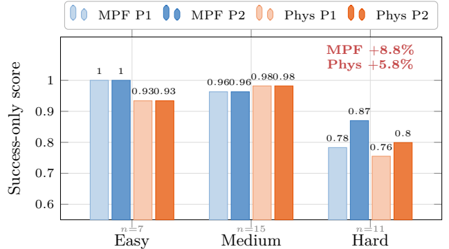
Figure 9: Paired KG growth comparison: success-only MPF and physics score for the same tasks run in pass 1 (0 prior Run nodes) vs. pass 2 (50 prior Run nodes). Only tasks succeeding in both passes are compared ( n=33 ; novel tasks omitted as they rely on pre-seeded material definitions). Easy and medium tasks are at ceiling; hard tasks gain +8.8% MPF and +5.8% physics score , the category where similarity-based warm-start adds most value.
