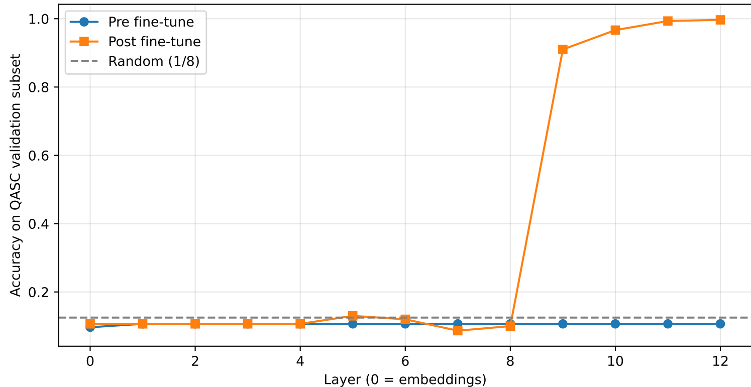
Per-layer answer accuracy via logit lens (gpt2)
