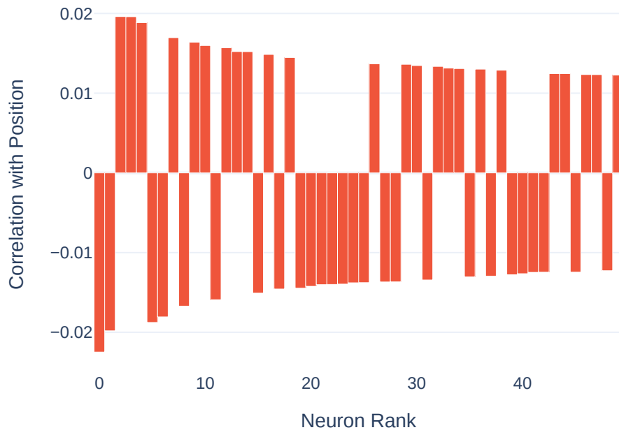
Top 50 Neurons
