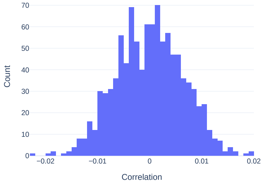
Correlation Distribution
