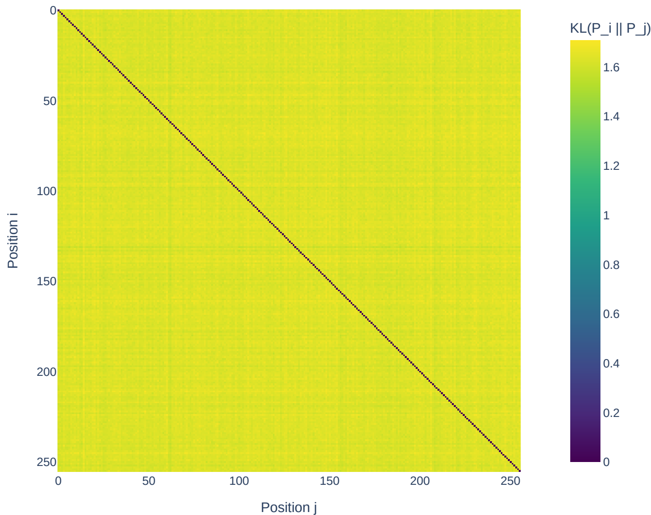
Position Distinguishability (KL Divergence)
