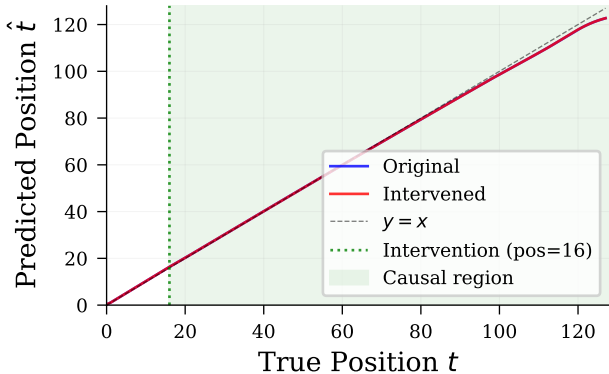
K = 16 : Predictions
