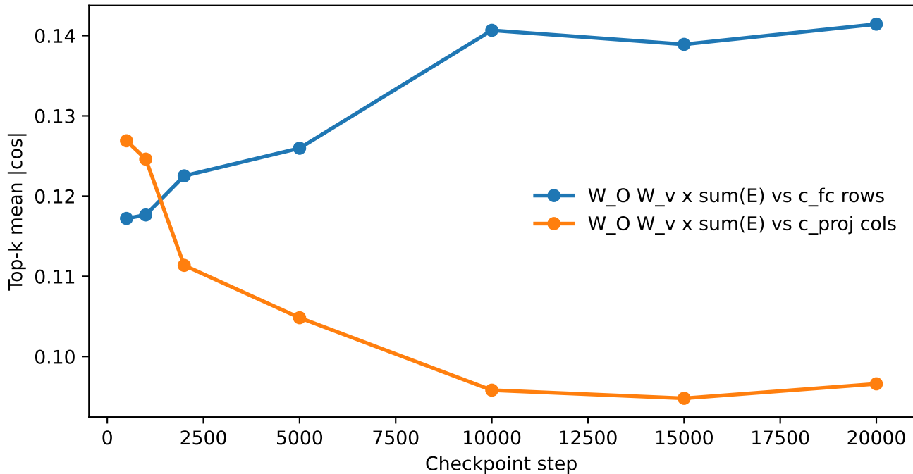
Decoding Vector Alignment with W_O (top-k mean |\cos| )
