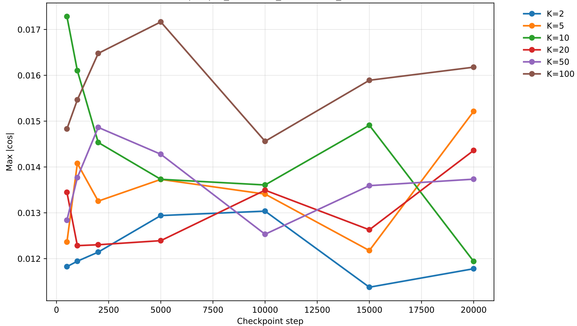
Max |\cos| W_V \cdot \text{sum}(E_k) vs MLP c_{fc} rows
