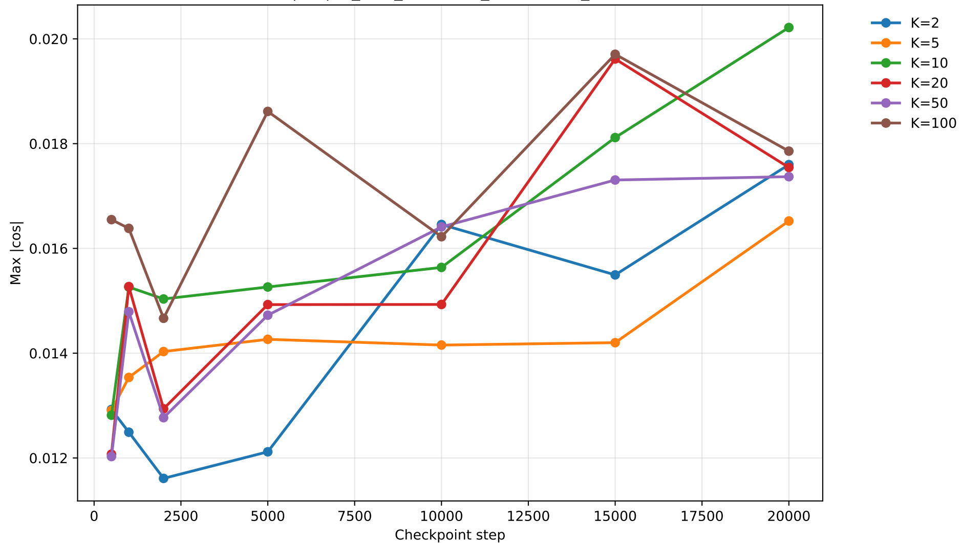
Max |\cos| W_O W_V \cdot \text{sum}(E_k) vs MLP c_fc rows
