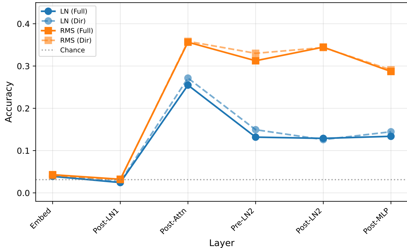
Trained Initialization
