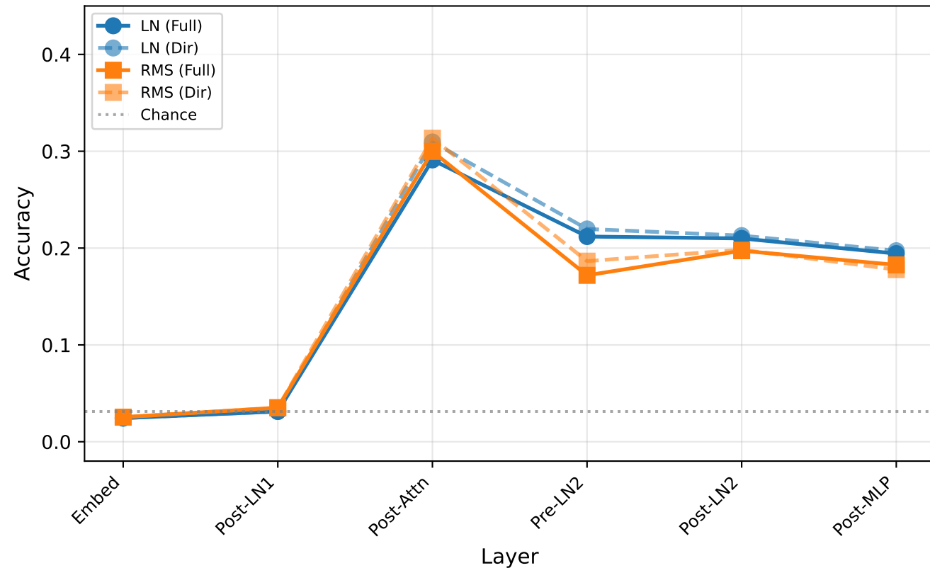
Random Initialization
