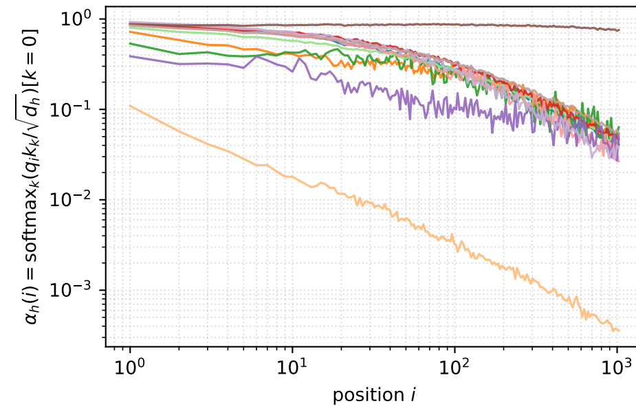
ATTN2-12H, L = 1024
