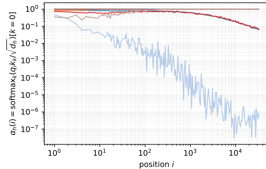
ATTN2-12H, L = 32768
