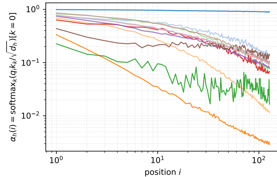
ATTN2-12H, L = 128
