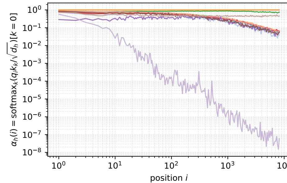
ATTN2-12H, L = 8192
