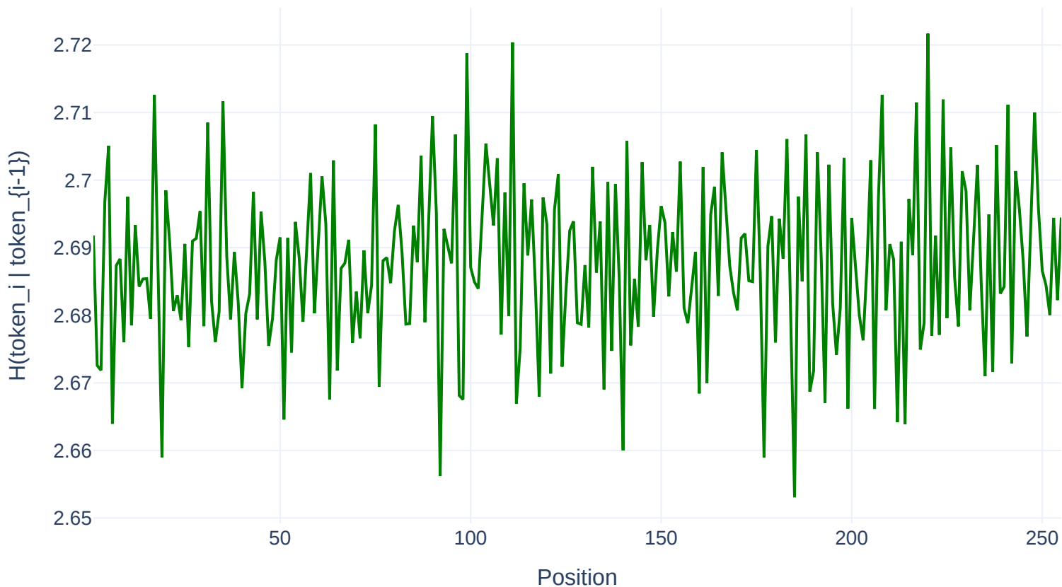
Token Transition Entropy by Position
