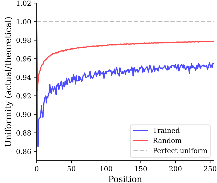
B) Both models near-uniform (Trained: 94.26%, Random: 97.34%)
