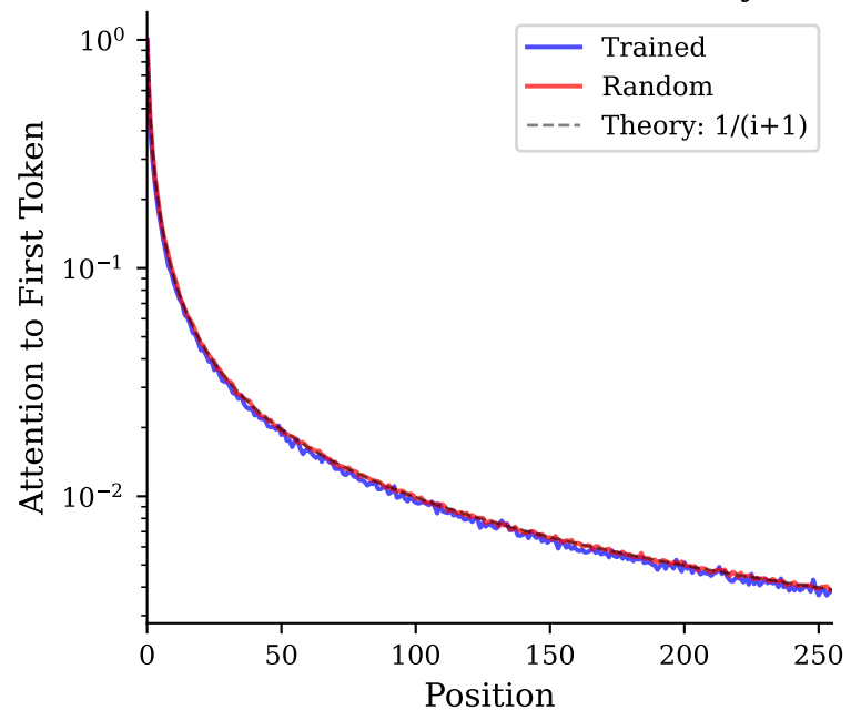
C) First-token attention decay
