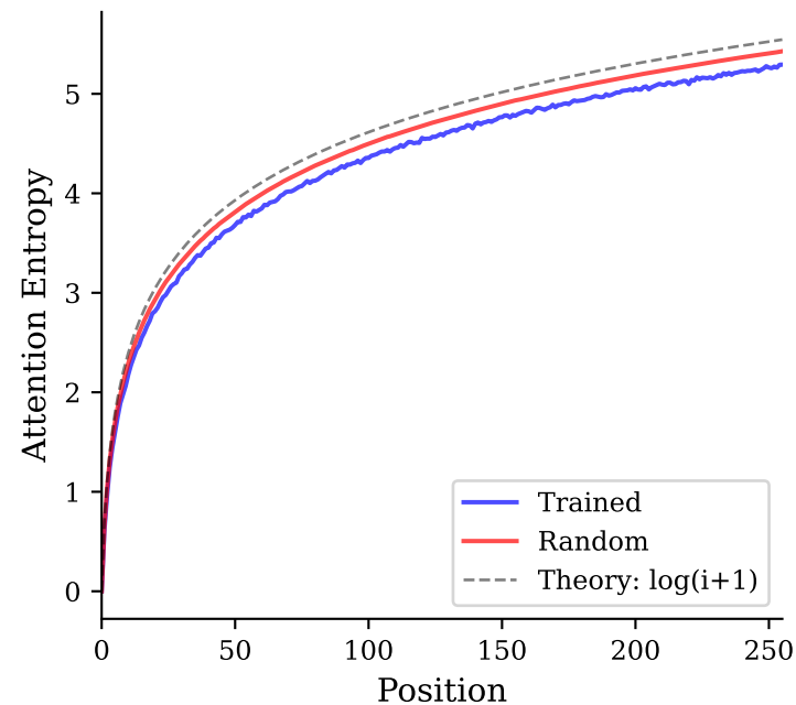
A) Entropy follows theory (Trained r=0.9998 )
