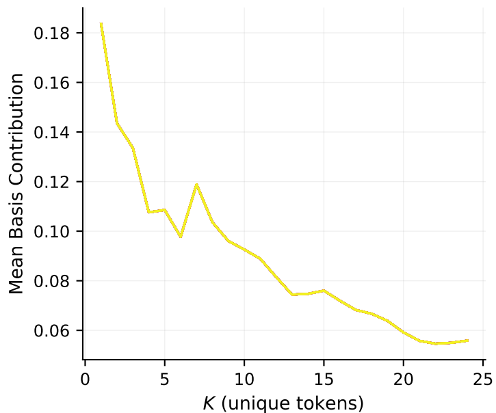
Post-Attention
