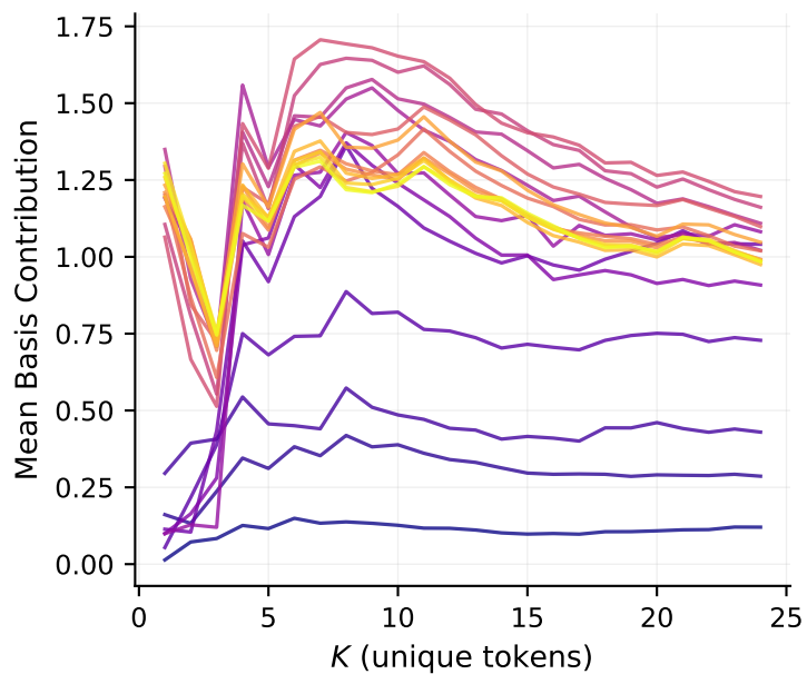
Post-MLP
