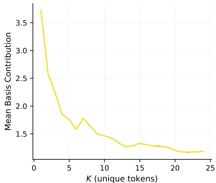
Post-LN2
